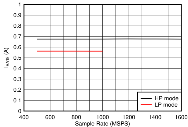
Low power background calibration mode, independent of JMODE Figure 5-83. Quad Channel, I_{VA19} vs F_S
