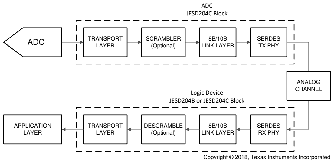
Figure 6-5. Simplified 8B/10B Encoded JESD204C Interface Diagram
