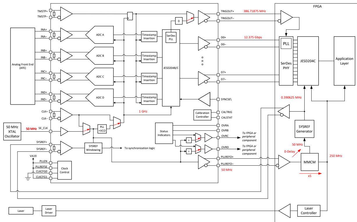
Figure 7-1. Typical Configuration for a LiDAR Digitizer
