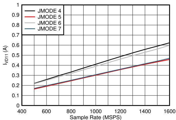
Figure 5-86. Quad Channel, I_{VD11} vs F_S and JMODE 4 - 7
