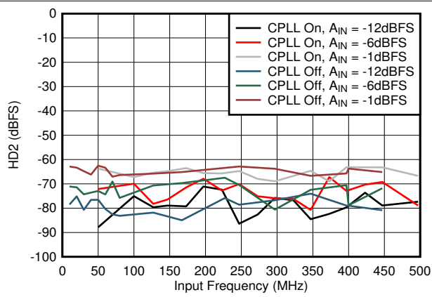
Figure 5-58. HD2 vs A_{IN} and C-PLL
