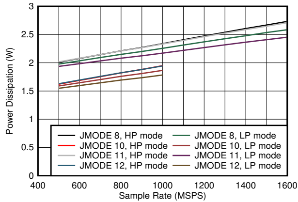
Low power background calibration mode Figure 5-81. Quad Channel, Power Dissipation vs F_S and JMODE 8 - 12
