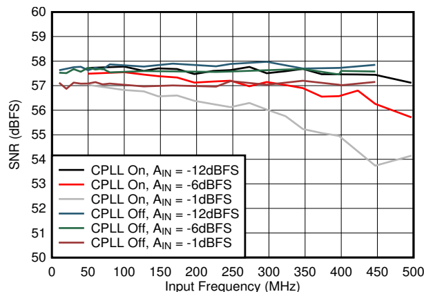
Figure 5-55. SNR vs A_{IN} and C-PLL
