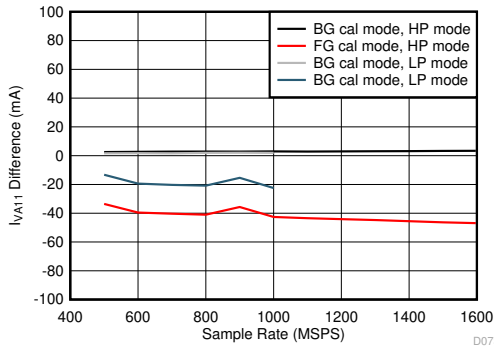
Figure 5-117. Single Channel, I_{VA11} Change with Calibration Mode
