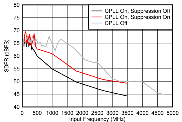
Figure 5-40. SFDR vs F_{IN} and C-PLL modes
