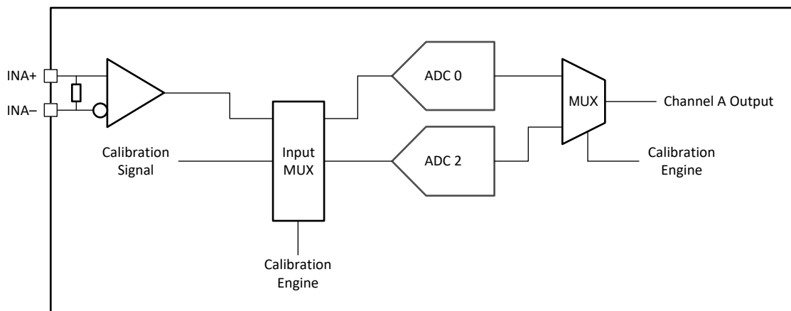
Figure 6-15. Single Channel Calibration System Block Diagram
