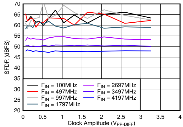
Figure 5-36. SFDR vs A_{CLK}
