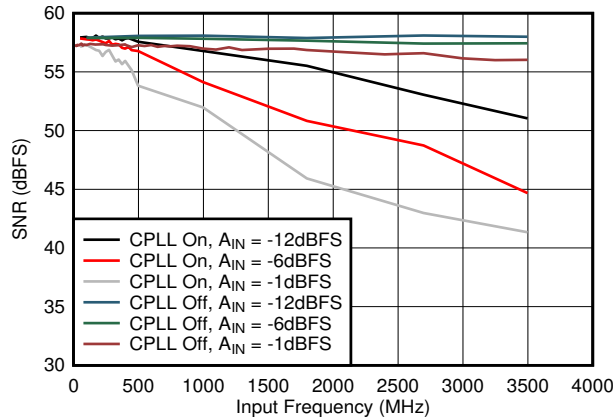
Figure 5-49. SNR vs A_{IN} and C-PLL
