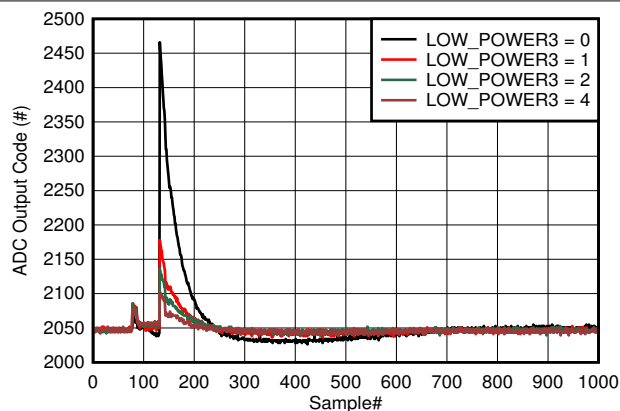
Figure 6-10. Background Calibration Core Transition In Low Power Mode
