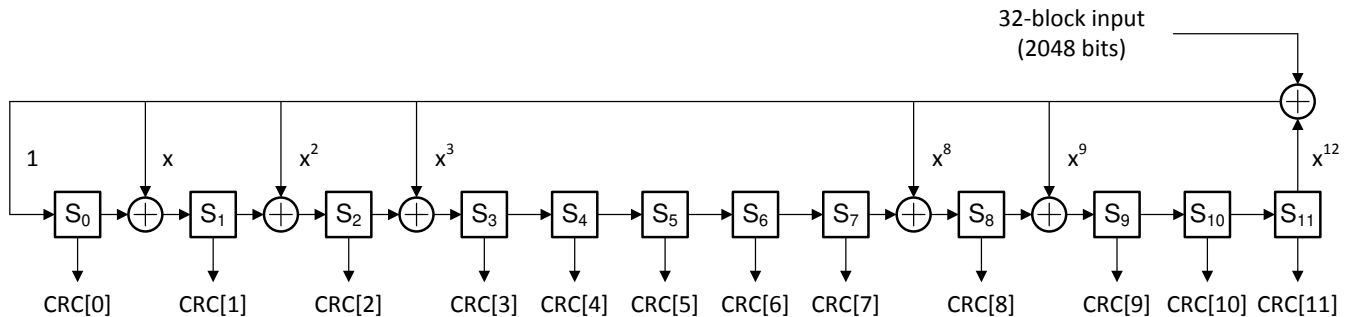
Figure 6-7. CRC-12 Parity Bit Generator
