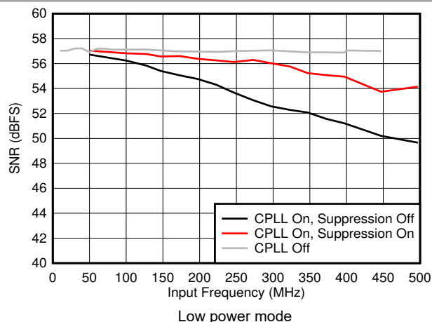
Figure 5-45. SNR vs F_{IN} and C-PLL modes
