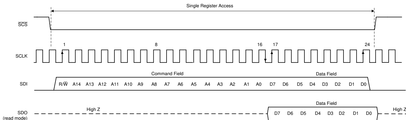
Figure 6-16. Serial Interface Protocol: Single Read/Write
