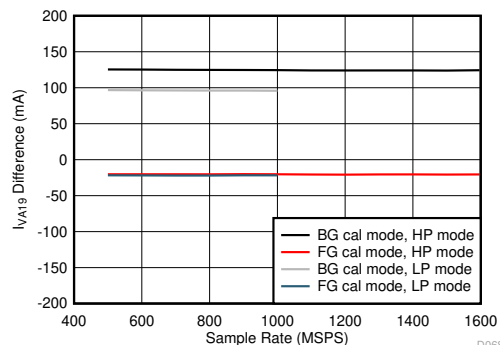
Figure 5-112. Quad Channel, I_{VA19} Change with Calibration Mode
