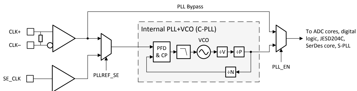
Figure 6-4. Converter PLL (C-PLL) Architecture
