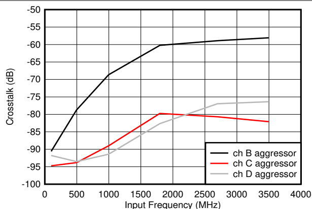
Figure 5-77. Crosstalk to Channel A vs F_{IN}
