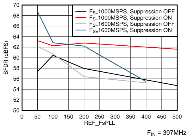
Figure 5-39. SFDR vs F_{REF} and Suppression
