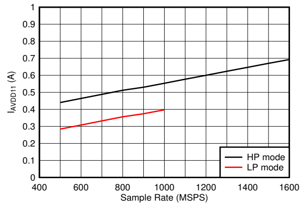
Low power background calibration mode, independent of JMODE Figure 5-84. Quad Channel, I_{VA11} vs F_S
