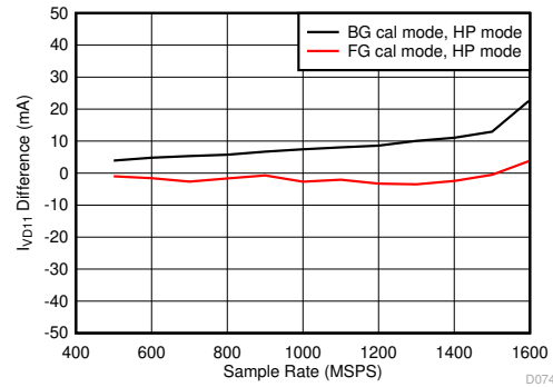
Figure 5-118. Quad Channel, I_{VD11} Change with Calibration Mode
