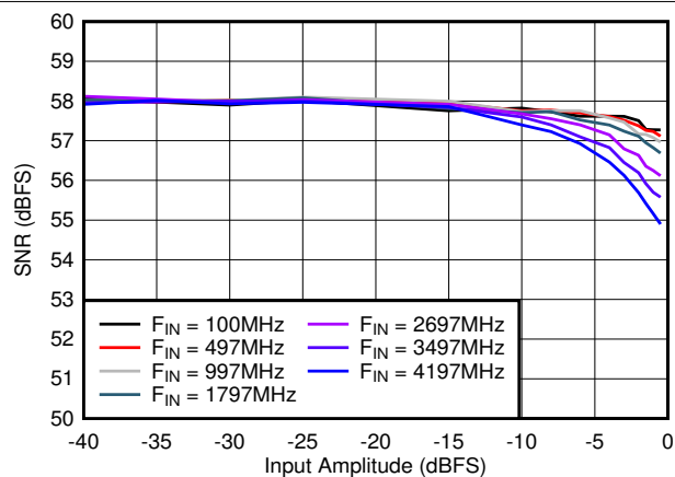
Figure 5-33. SNR vs A_{IN}
