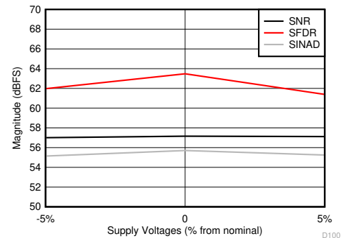
All supplies changed together, high power mode Figure 5-60. SNR, SFDR and SINAD vs Supply Voltage
