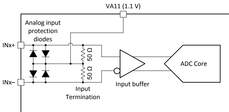
Figure 6-2. Analog Input Internal Termination and Protection Diagram
