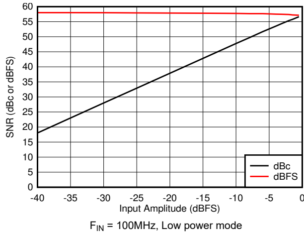
Figure 5-35. SNR vs A_{IN}
