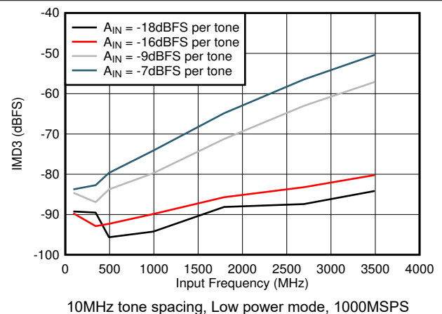
Figure 5-76. IMD3 vs F_{IN}
