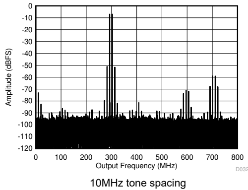
Figure 5-71. Two Tone FFT at 3498MHz
