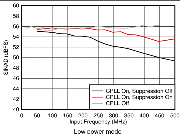
Figure 5-46. SINAD vs F_{IN} and C-PLL modes
