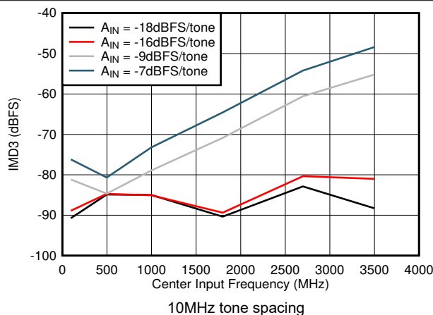
Figure 5-75. IMD3 vs F_{IN}
