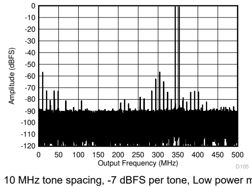
Figure 5-72. Two Tone FFT at 348 MHz
