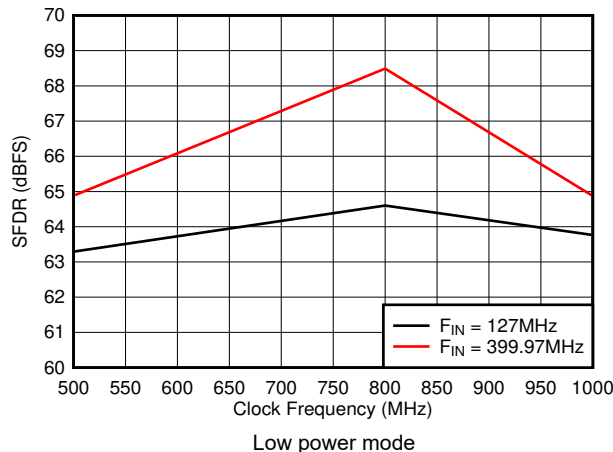
Figure 5-29. SFDR vs Sample Rate
