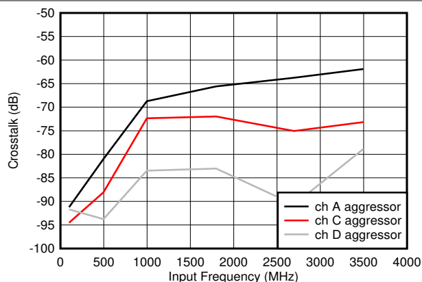
Figure 5-78. Crosstalk to Channel B vs F_{IN}
