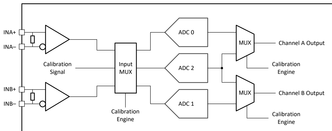
Figure 6-14. DualChannel Calibration System Block Diagram
