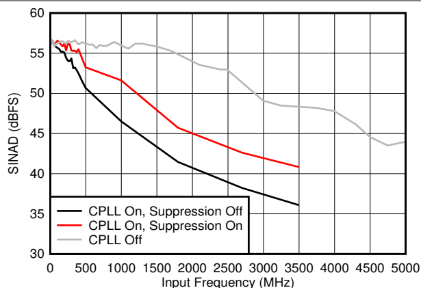
Figure 5-42. SINAD vs F_{IN} and C-PLL modes
