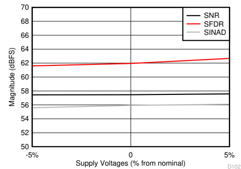
All supplies changed together, low power mode, F_S = 1000 MSPS Figure 5-62. SNR, SFDR and SINAD vs Supply Voltages
