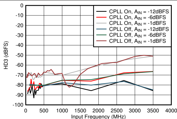
Figure 5-53. HD3 vs A_{IN} and C-PLL
