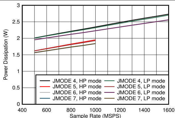
Figure 5-80. Quad Channel, Power Dissipation vs F_S and JMODE 4 - 7
