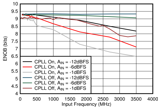
Figure 5-51. ENOB vs A_{IN} and C-PLL
