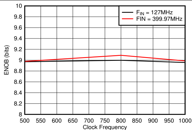
Figure 5-31. ENOB vs Sample Rate
