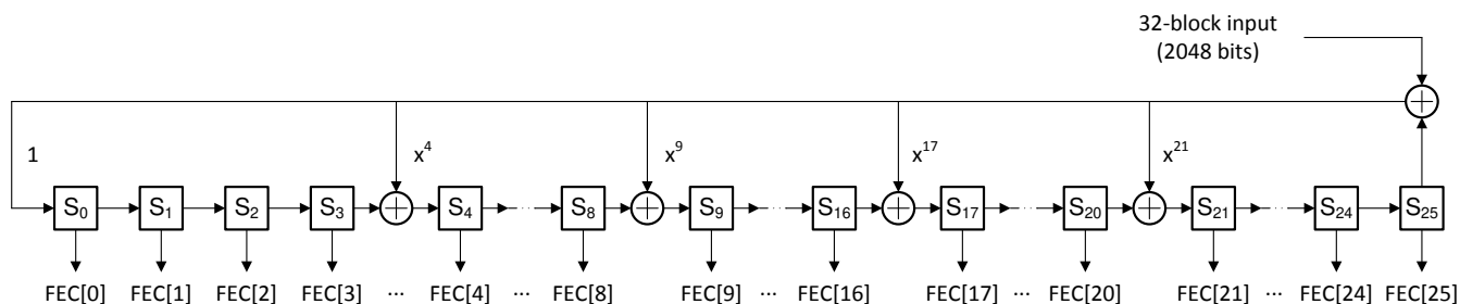
Figure 6-8. FEC Parity Bit Generator
