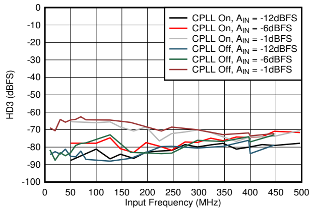
Figure 5-59. HD3 vs A_{IN} and C-PLL
