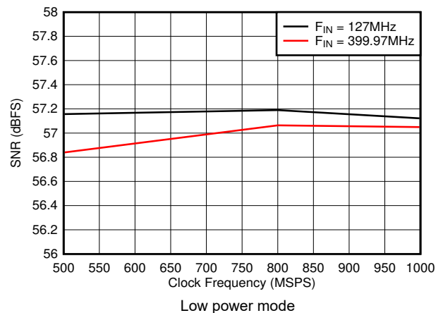
Figure 5-28. SNR vs Sample Rate
