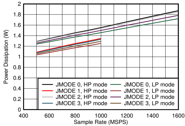
Figure 5-89. Dual Channel, Power Dissipation vs F_S and JMODE 0 - 3
