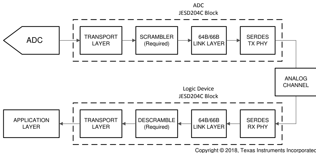
Figure 6-6. Simplified 64B/66B Encoded JESD204C Interface Diagram
