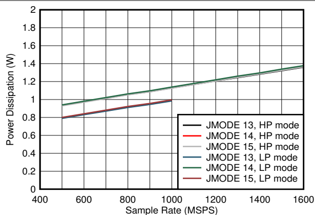
Figure 5-102. Single Channel, Power Dissipation vs F_S and JMODE 13 - 15
