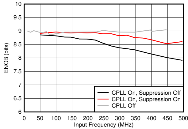
Figure 5-47. ENOB vs F_{IN} and C-PLL modes
