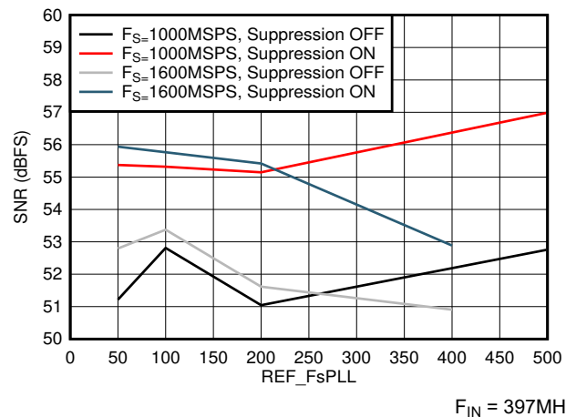
Figure 5-38. SNR vs F_{REF} and Suppression
