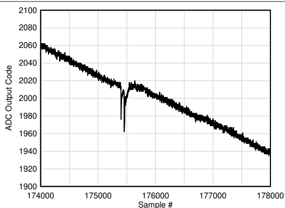
Figure 5-127. Background Calibration Core Transition (AC Signal Zoomed)
