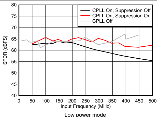
Figure 5-44. SFDR vs F_{IN} and C-PLL modes
