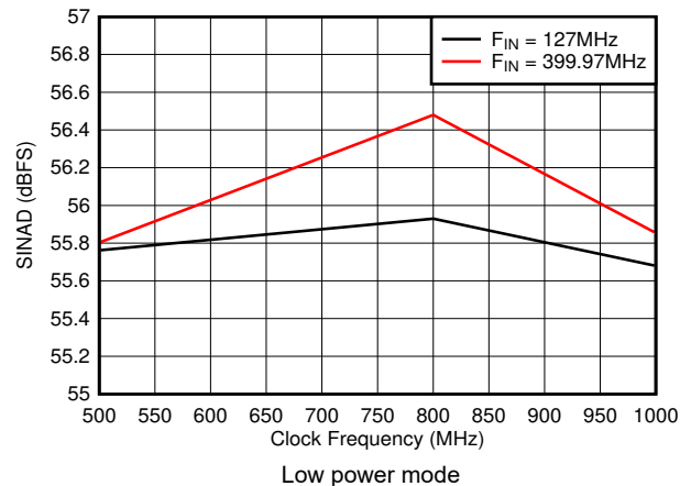
Figure 5-30. SINAD vs Sample Rate
