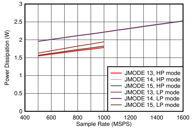
Low power background calibration mode Figure 5-82. Quad Channel, Power Dissipation vs F_S and JMODE 13 - 15
