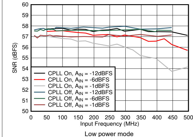
Figure 5-55. SNR vs A_{IN} and C-PLL
