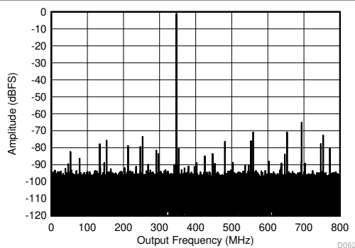
High power mode, C-PLL on Figure 5-5. Single Tone FFT at 347 MHz and -1 dBFS
