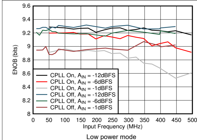
Figure 5-57. ENOB vs A_{IN} and C-PLL
