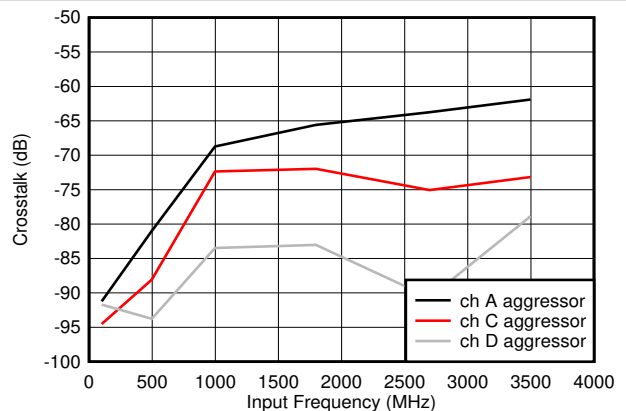
Figure 7-78. Crosstalk to Channel B vs F_{IN}
