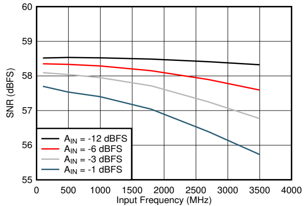
Figure 5-18. SNR vs Input Frequency
