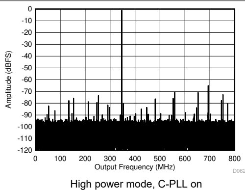
Figure 5-5. Single Tone FFT at 347MHz and -1dBFS
