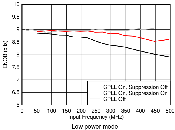
Figure 5-47. ENOB vs F_{IN} and C-PLL modes
