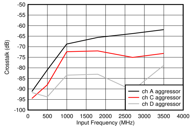
Figure 5-78. Crosstalk to Channel B vs F_{IN}
