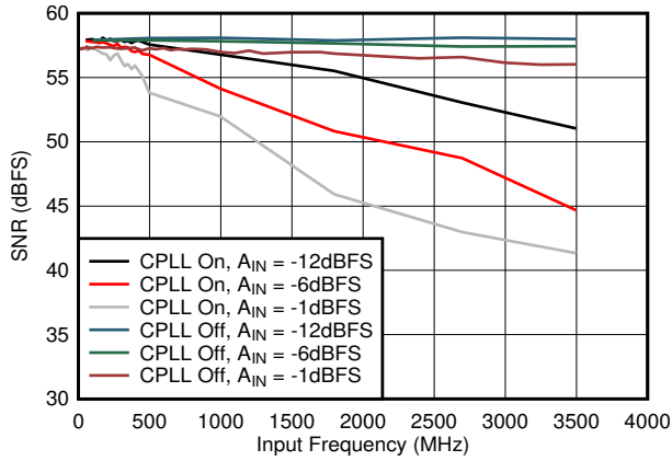
Figure 5-49. SNR vs A_{IN} and C-PLL
