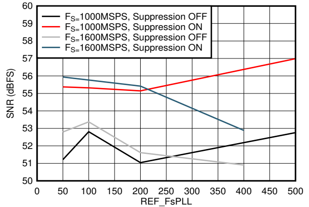
Figure 5-38. SNR vs F REF and Suppression
