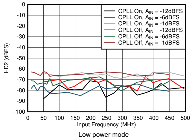
Figure 5-58. HD2 vs A_{IN} and C-PLL
