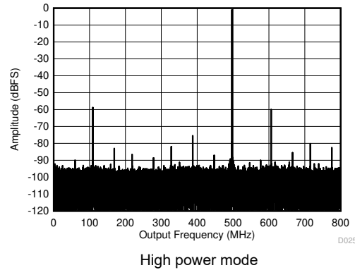
Figure 5-10. Single Tone FFT at 2097MHz and -1dBFS
