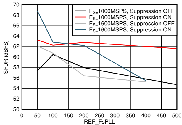
Figure 5-39. SFDR vs F REF and Suppression
