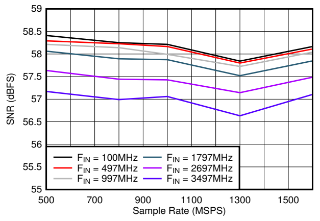
Figure 5-24. SNR vs Sample Rate
