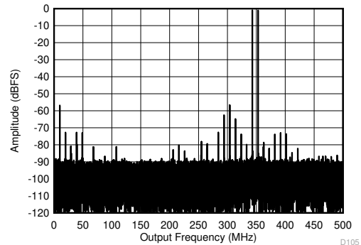
Figure 5-70. Two Tone FFT at 1798MHz
