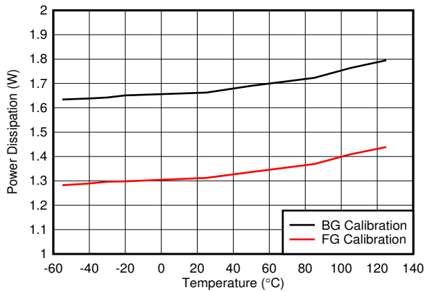
Figure 5-123. Single Channel, Power Dissipation vs Temperature
