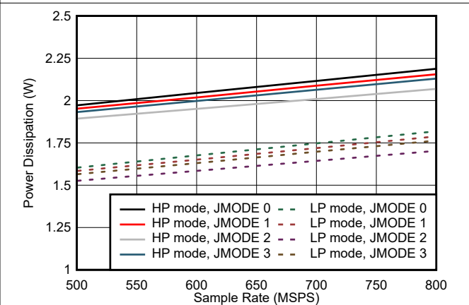
Figure 5-74. Quad Channel, Power Dissipation vs F_S for JMODES 0 - 3
