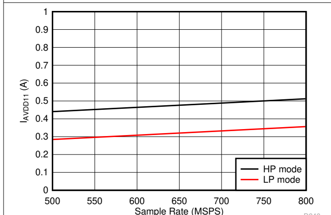
Figure 5-79. Quad Channel, I_{VA11} vs F_S
