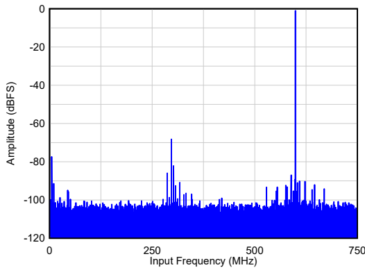
SNR = 66.8 dBFS, HD23 = 67 dBc, Non HD23 = 82 dBFS A_{IN} = -1\text{ dBFS} , 4x AVG, Dither = DIS
