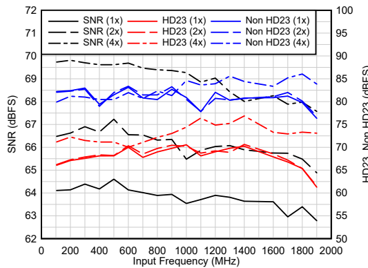
A_{IN} = -1\text{ dBFS} , Dither = DIS
