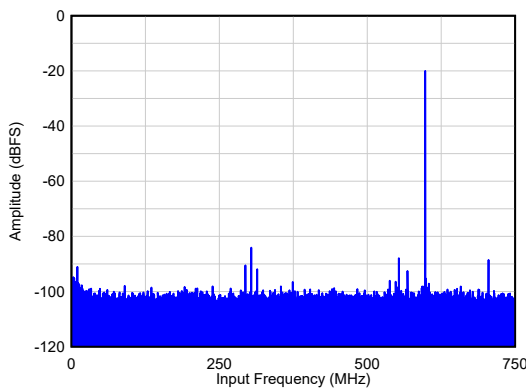
SNR = 65.2 dBFS, HD23 = 64 dBc, Non HD23 = 88 dBFS A_{IN} = -20\text{ dBFS} , 1x AVG, Dither = DIS
