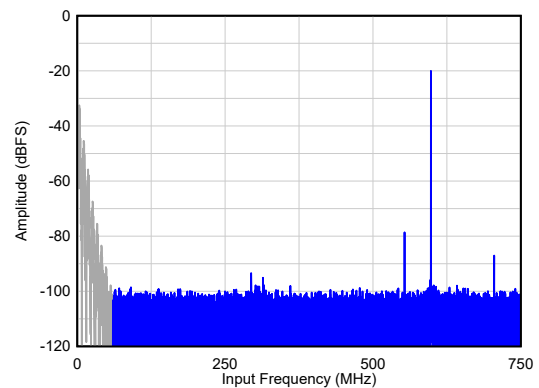
SNR = 64.8 dBFS 1 , HD23 = 59 dBc, Non HD23 = 79 dBFS A_{IN} = -20\text{ dBFS} , 1x AVG, Dither = EN
