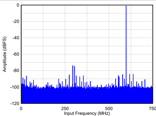
Figure 6-3. Single Tone FFT at F_{IN} = 600\text{ MHz}
