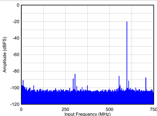
SNR = 67.9 dBFS, HD23 = 64 dBc, Non HD23 = 86 dBFS A_{IN} = -20\text{ dBFS} , 2x AVG, Dither = DIS
