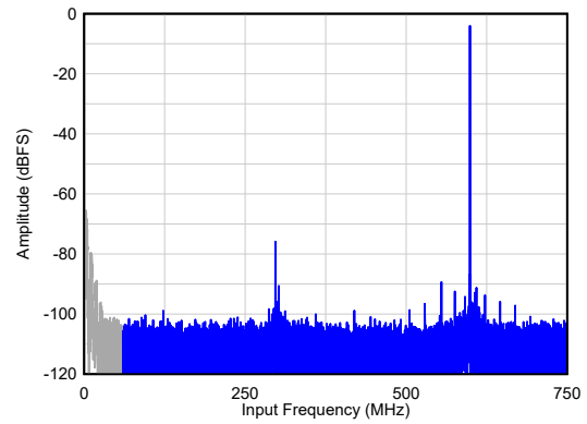
SNR = 67.0 dBFS 1 , HD23 = 75 dBc, Non HD23 = 89 dBFS A_{IN} = -4\text{ dBFS} , 4x AVG, Dither = EN
