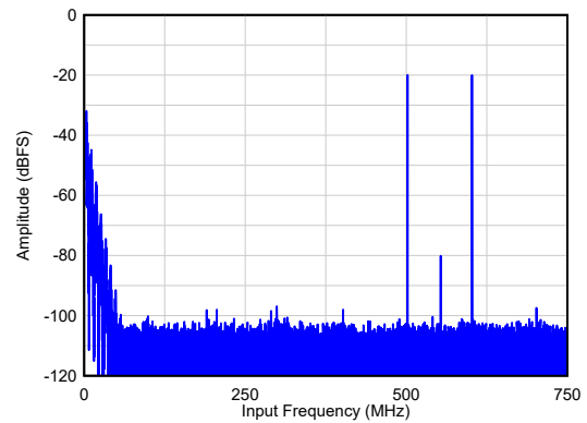
IMD3 = 77 dBc A_{IN} = -20\text{ dBFS/tone} , 2x AVG, Dither = EN
