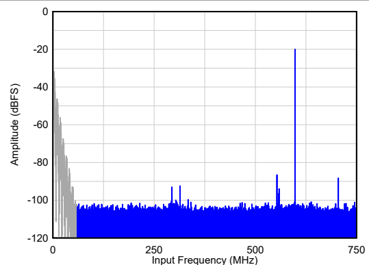
SNR = 67.6 dBFS 1 , HD23 = 67 dBc, Non HD23 = 87 dBFS A_{IN} = -20\text{ dBFS} , 2x AVG, Dither = EN
