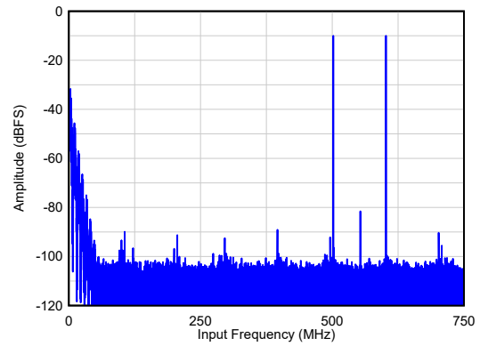
IMD3 = 79 dBc A_{IN} = -10\text{ dBFS/tone} , 2x AVG, Dither = EN
