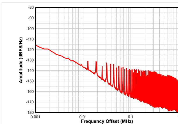
Figure 7-6. Dither Close-Up
