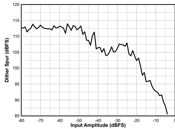
F_{IN} = 900 MHz,
