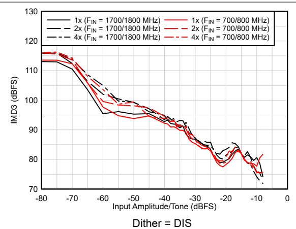
Figure 6-34. IMD3 Performance vs A_{IN}
