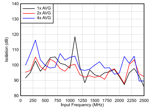
Figure 6-42. Isolation vs Input Frequency
