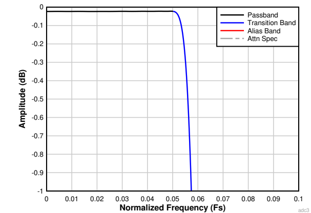
Figure 7-27. Decimation by 8 Passband Ripple Response
