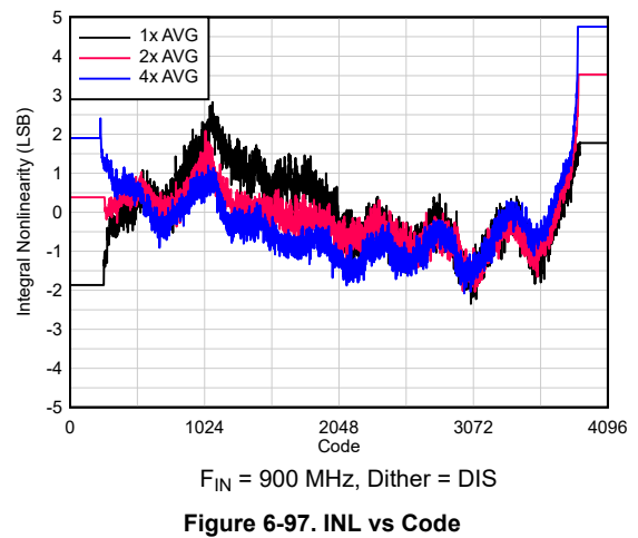
Figure 6-97. INL vs Code
