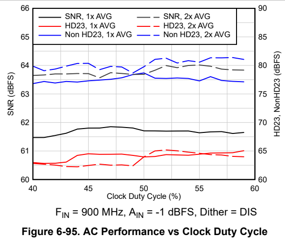
Figure 6-95. AC Performance vs Clock Duty Cycle
