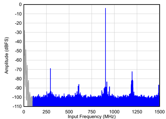
SNR = 60.9 dBFS 1 , SFDR = 64 dBc, Non HD23 = 82 dBFS A_{IN} = -4 dBFS, 1x AVG, Dither = EN
