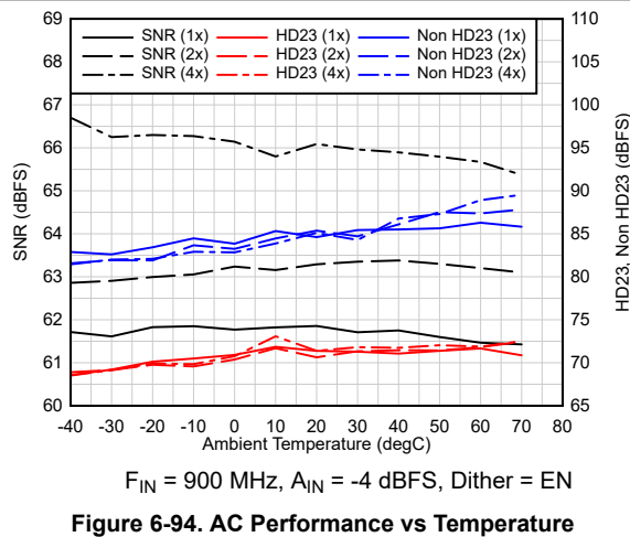
Figure 6-94. AC Performance vs Temperature
