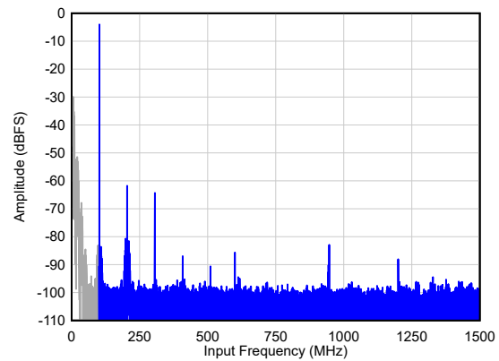
SNR = 61.7 dBFS 2 , SFDR = 58 dBc, Non HD23 = 83 dBFS A_{IN} = -4 dBFS, 1x AVG, Dither = EN
