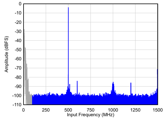
SNR = 61.8 dBFS 1 , SFDR = 68 dBc, Non HD23 = 84 dBFS A_{IN} = -4 dBFS, 1x AVG, Dither = EN
