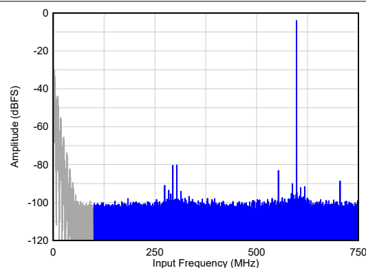
Figure 6-4. Single Tone FFT at F_{IN} = 600\text{ MHz}
