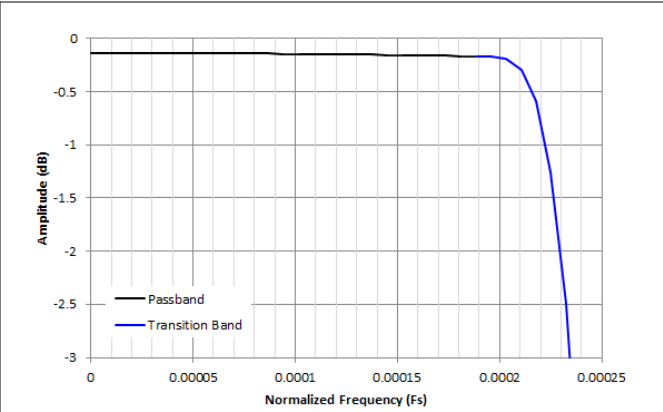
Figure 8-44. Decimation by 2048 Passband Ripple Response
