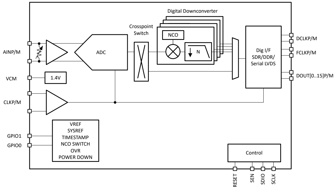
Figure 8-1. Block Diagram
