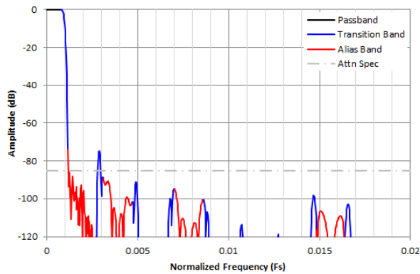
Figure 8-39. Complex Decimation by 512 Filter Response
