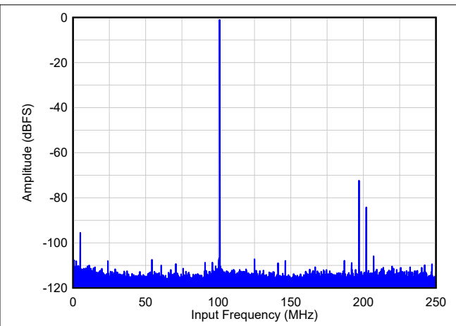
Figure 8-69. FFT: F_{IN} = 105\text{MHz} , low latency mode
