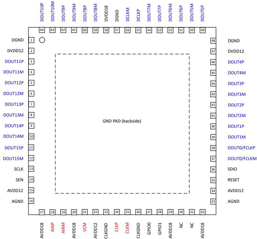
Figure 5-1. RTD Package, 64 Pin VQFN (Top View)
