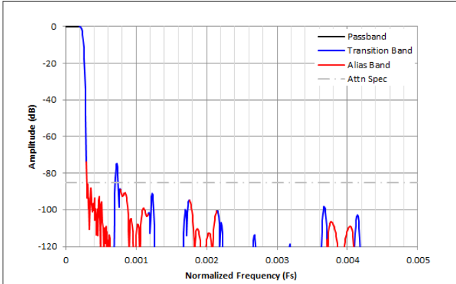
Figure 8-43. Complex Decimation by 2048 Filter Response
