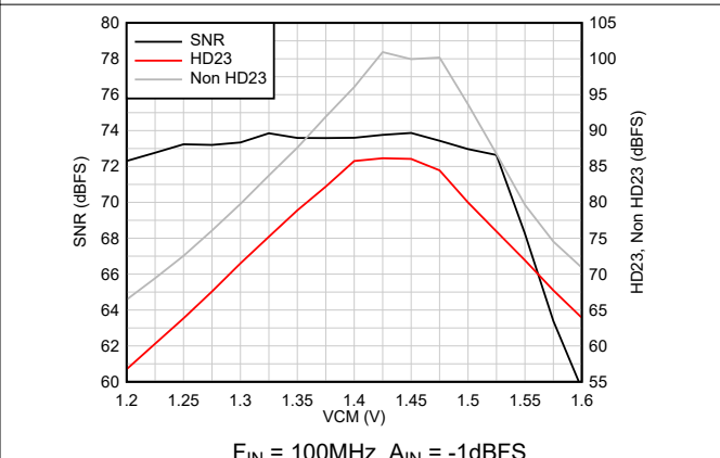
Figure 6-48. AC Performance vs VCM
