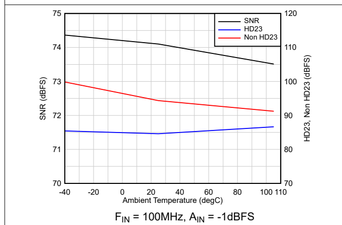
Figure 6-49. AC Performance vs Temperature
