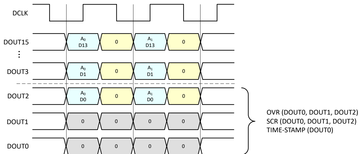
Figure 8-56. Output data format in DDR LVDS mode
