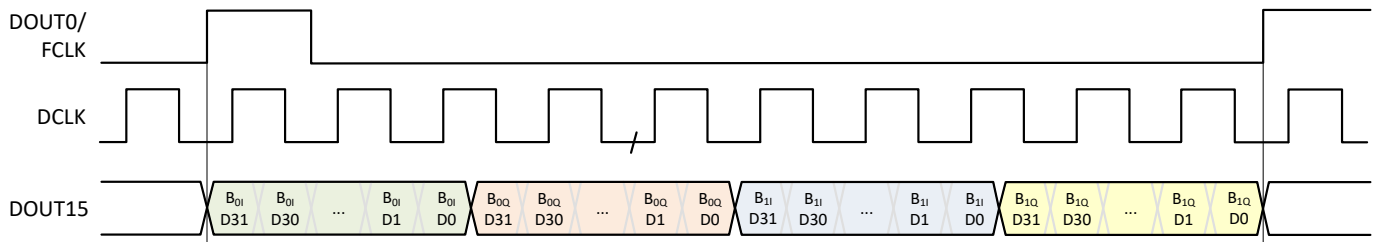
Figure 8-60. SLVDS frame assembly for example 4
