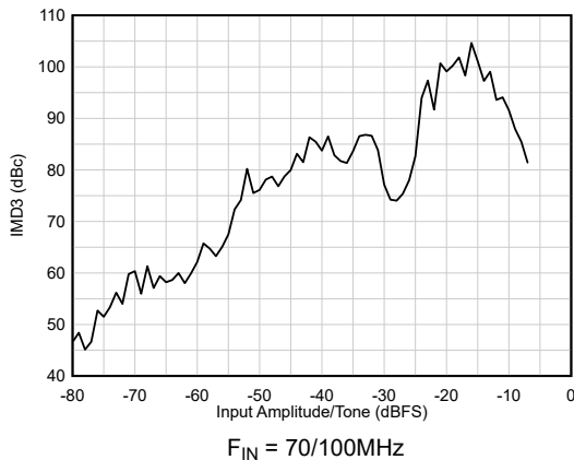
Figure 6-17. IMD3 vs A_{IN}
