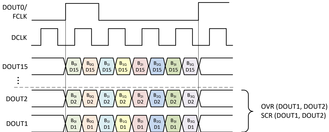
Figure 8-61. Output Data Substitution: 16 SLVDS Lanes
