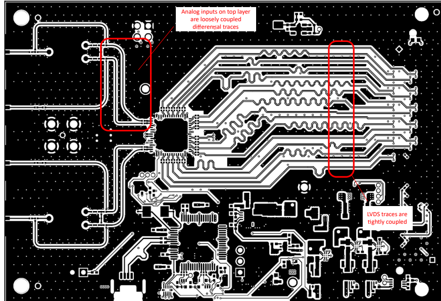
Figure 9-11. Layout example: top layer of ADC366x EVM
