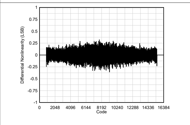
Figure 6-50. DNL
