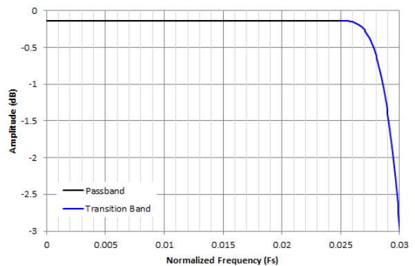
Figure 8-30. Decimation by 16 Passband Ripple Response
