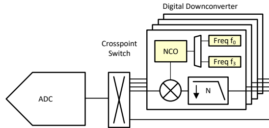
Figure 8-53. NCO Block Diagram
