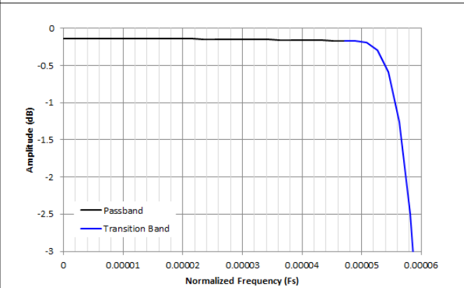
Figure 8-48. Decimation by 8192 Passband Ripple Response
