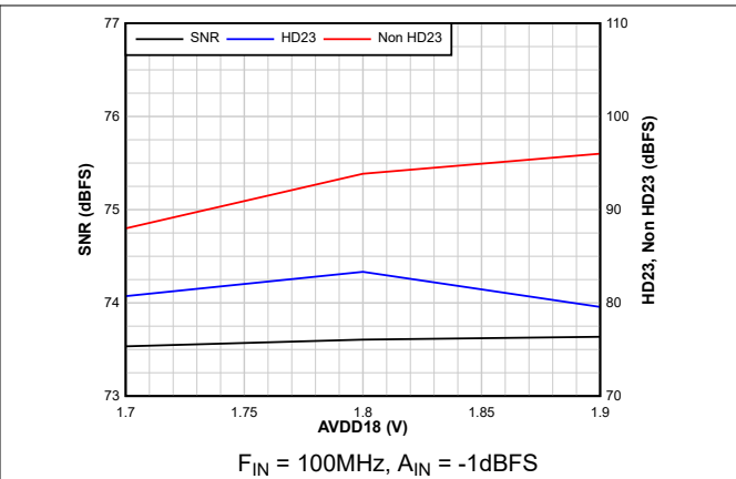
Figure 6-46. AC Performance vs AVDD18
