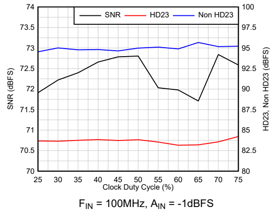
Figure 6-18. AC Performance vs Clock Duty Cycle
