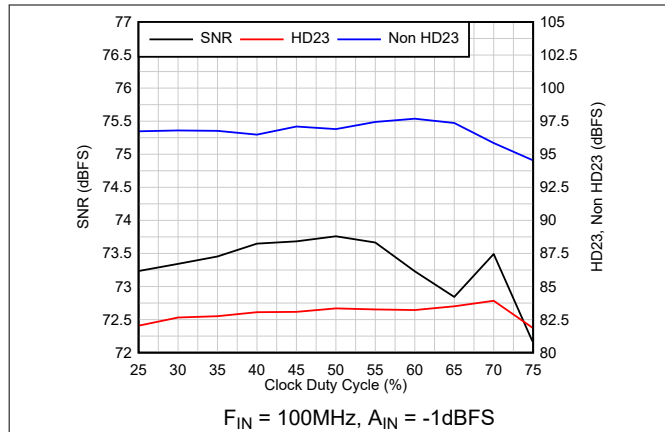
Figure 6-45. AC Performance vs Clock Duty Cycle
