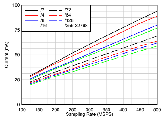
Figure 6-54. Current vs Sampling Rate
