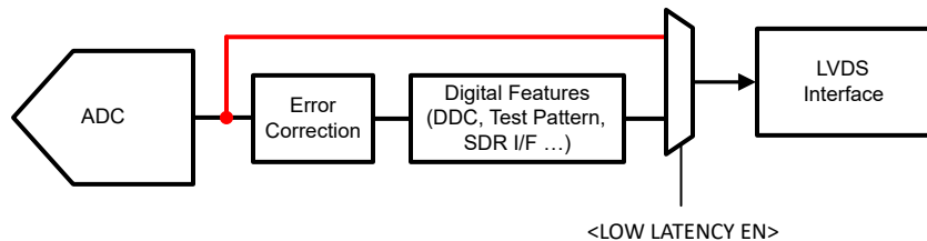
Figure 8-67. Low Latency Mode
