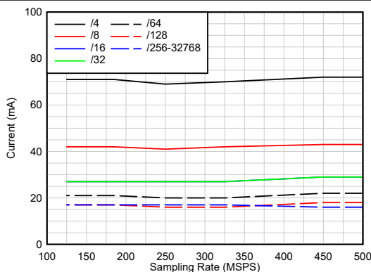
Complex Decimation, Quad Band, DVDD18 Figure 6-61. Current vs Sampling Rate
