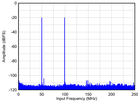
A_{IN} = -20\text{dBFS}/\text{tone} , \text{IMD3} = 97\text{dBc}
