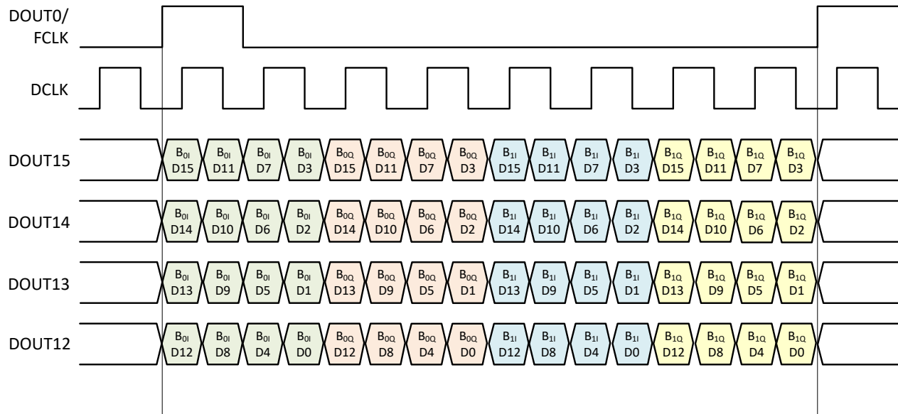
Figure 8-59. SLVDS frame assembly for example 3
