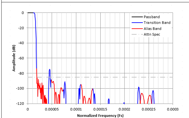
Figure 8-51. Complex Decimation by 32768 Filter Response
