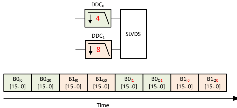
Figure 8-21. Unequal Decimation Factors
