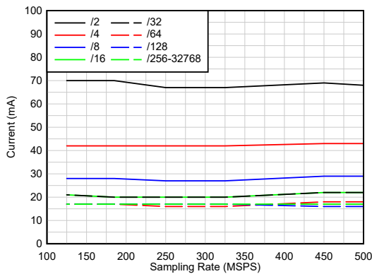
Complex Decimation, Dual Band, DVDD18 Figure 6-59. Current vs Sampling Rate
