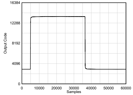
Figure 6-26. Pulse Response
