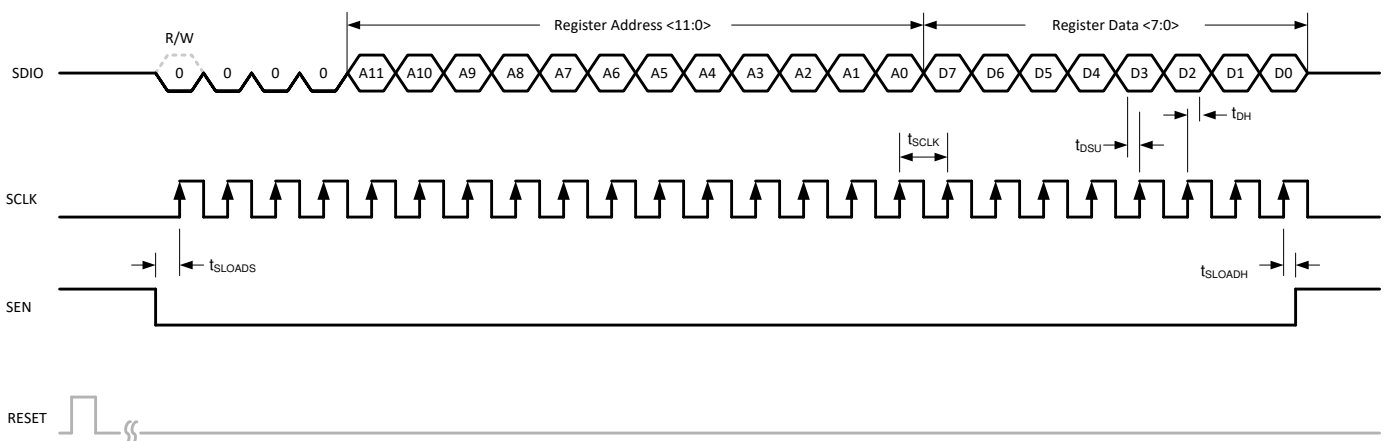
Figure 8-70. Serial Register Write Timing Diagram
