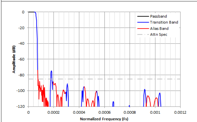
Figure 8-47. Complex Decimation by 8192 Filter Response
