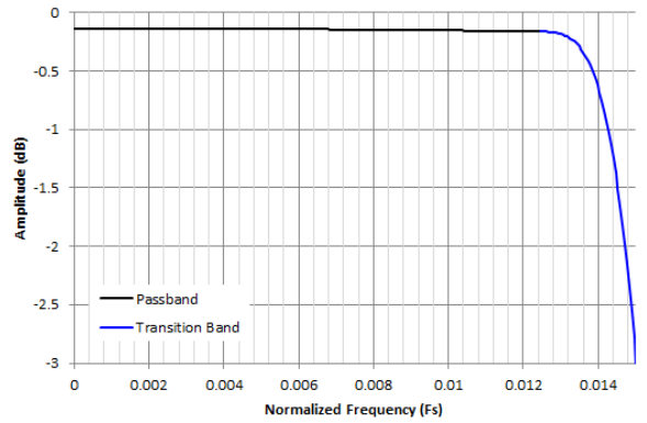
Figure 8-32. Decimation by 32 Passband Ripple Response
