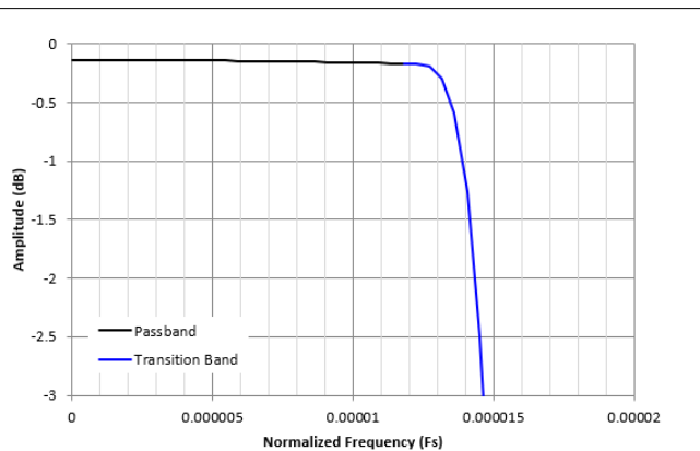
Figure 8-52. Decimation by 32768 Passband Ripple Response
