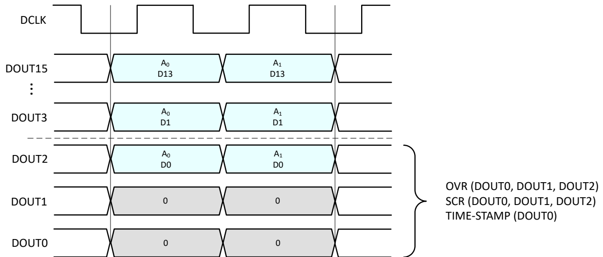
Figure 8-55. Output data format in SDR LVDS mode
