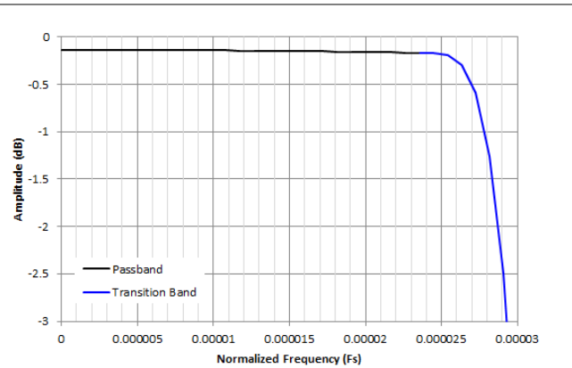
Figure 8-50. Decimation by 16384 Passband Ripple Response
