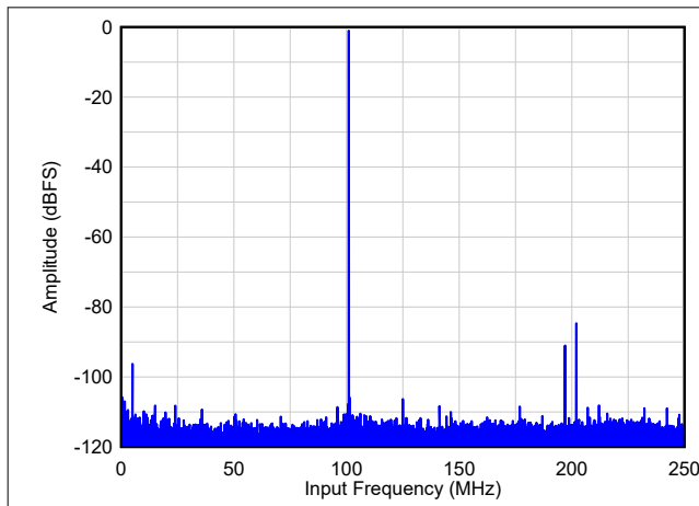
Figure 8-68. FFT: F_{IN} = 105\text{MHz} , normal mode
