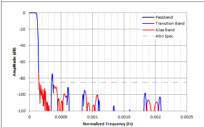
Figure 8-45. Complex Decimation by 4096 Filter Response
