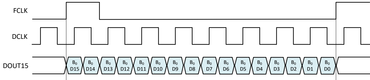
Figure 8-57. SLVDS frame assembly for example 1
