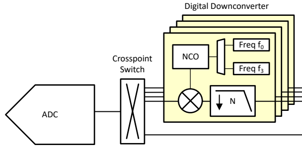
Internal digital down converter
