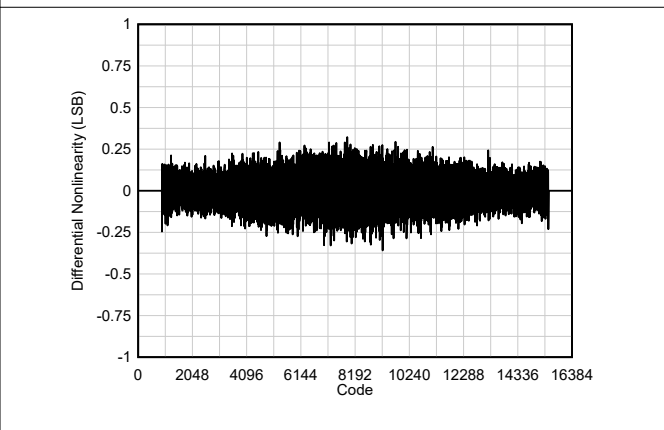
Figure 6-50. DNL
