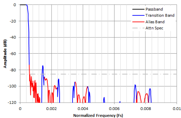
Figure 8-41. Complex Decimation by 1024 Filter Response
