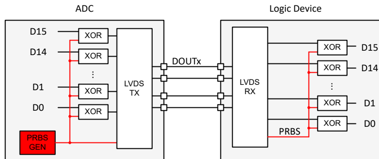
Figure 8-63. Output Scrambler
