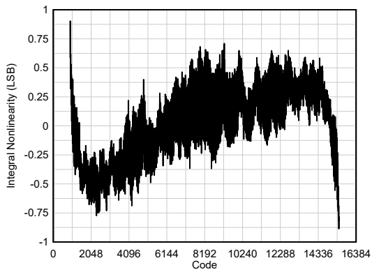
Figure 6-51. INL
