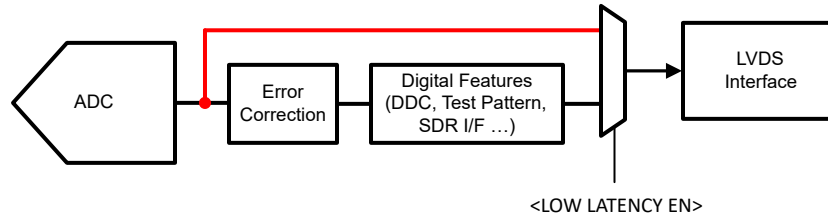
Figure 8-67. Low Latency Mode
