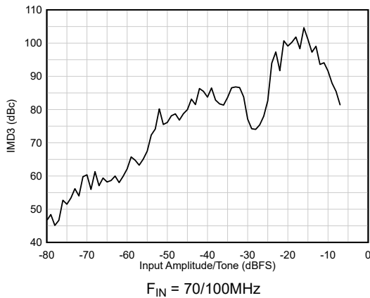
Figure 6-17. IMD3 vs A_{IN}
