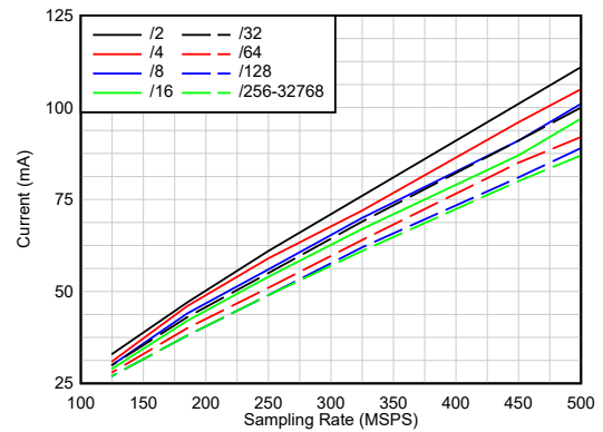
Complex Decimation, Single Band, DVDD12 Figure 6-58. Current vs Sampling Rate
