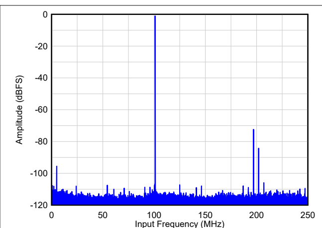
Figure 8-69. FFT: F_{IN} = 105\text{MHz} , low latency mode
