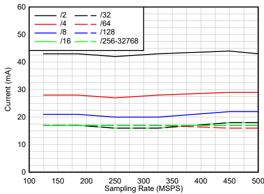
Complex Decimation, Single Band, DVDD18 Figure 6-57. Current vs Sampling Rate
