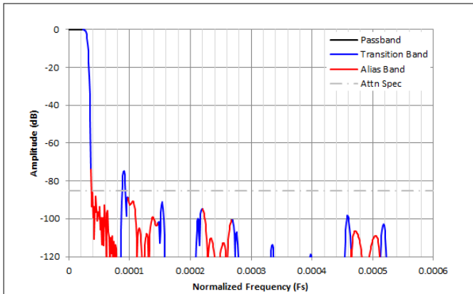
Figure 8-49. Complex Decimation by 16384 Filter Response
