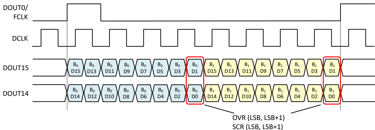
Figure 8-62. Output Data Substitution: <16 SLVDS Lanes
