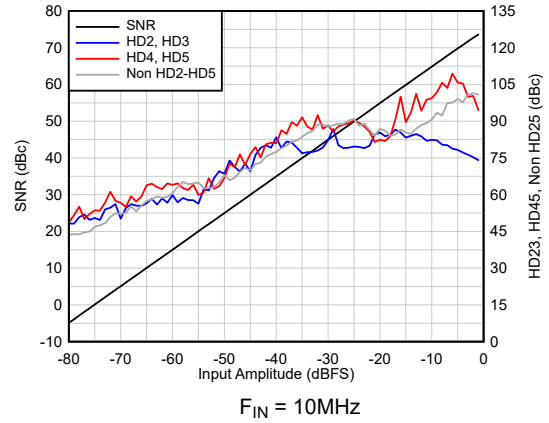
Figure 6-14. AC Performance vs A_{IN}
