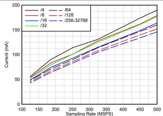
Complex Decimation, Quad Band, DVDD12 Figure 6-62. Current vs Sampling Rate
