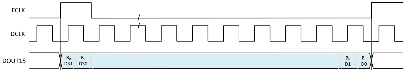
Figure 8-58. SLVDS frame assembly for example 2
