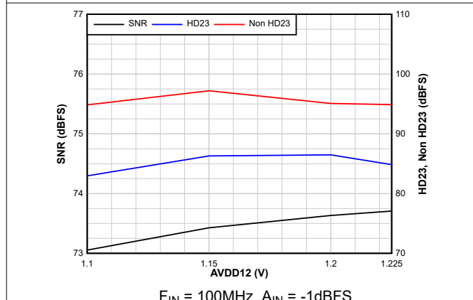
Figure 6-47. AC Performance vs AVDD12
