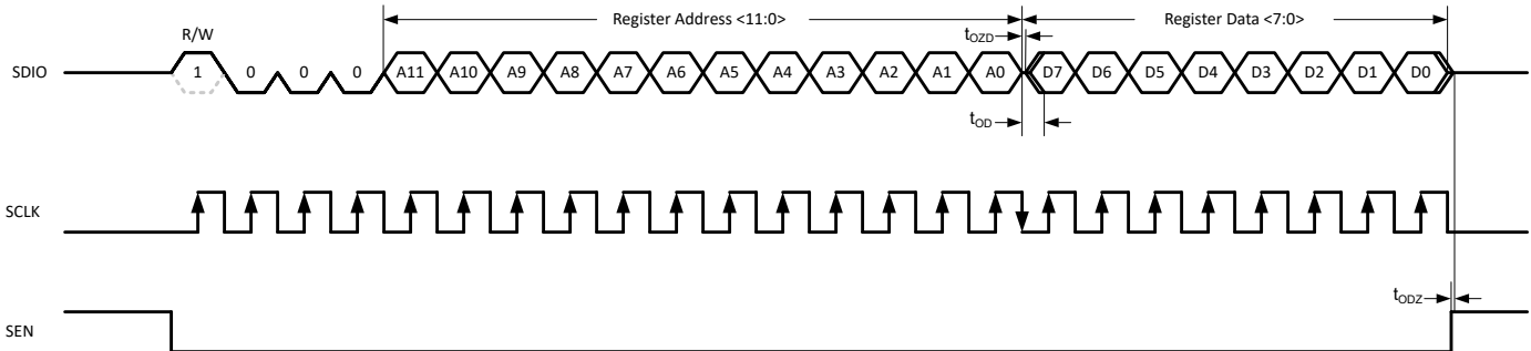
Figure 8-71. Serial Register Read Timing Diagram
