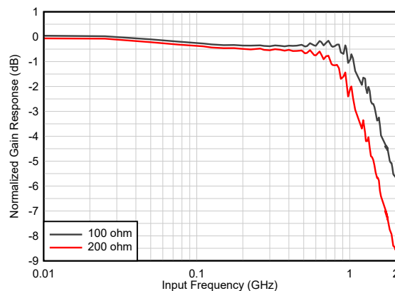
Figure 8-6. Full power input bandwidth for 100Ω and 200Ω internal termination
