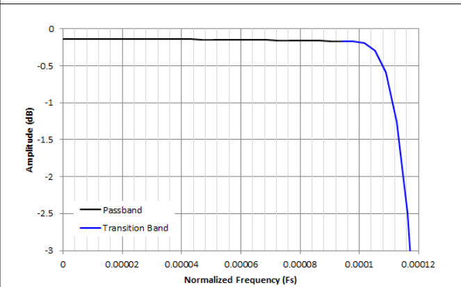
Figure 8-46. Decimation by 4096 Passband Ripple Response
