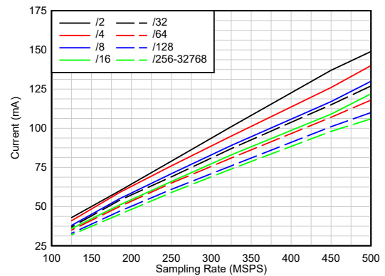
Complex Decimation, Dual Band, DVDD12 Figure 6-60. Current vs Sampling Rate
