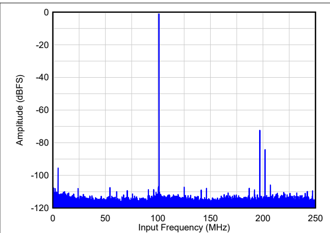
Figure 8-70. FFT: F_{IN} = 105\text{MHz} , low latency mode
