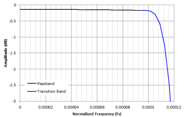
Figure 8-46. Decimation by 4096 Passband Ripple Response
