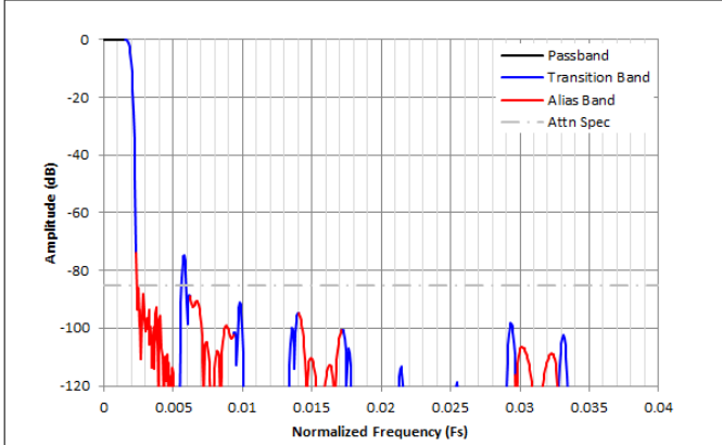
Figure 8-38. Complex Decimation by 256 Filter Response
