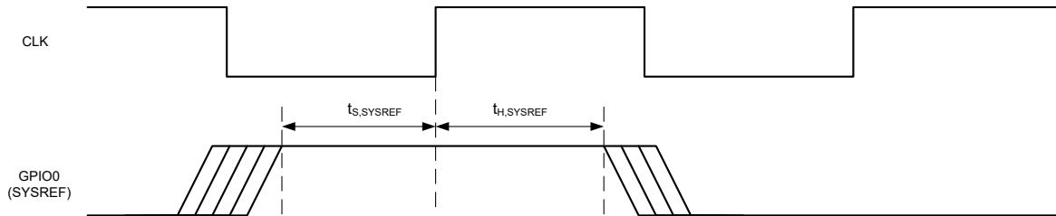
Figure 8-16. Timing: external synchronization input
