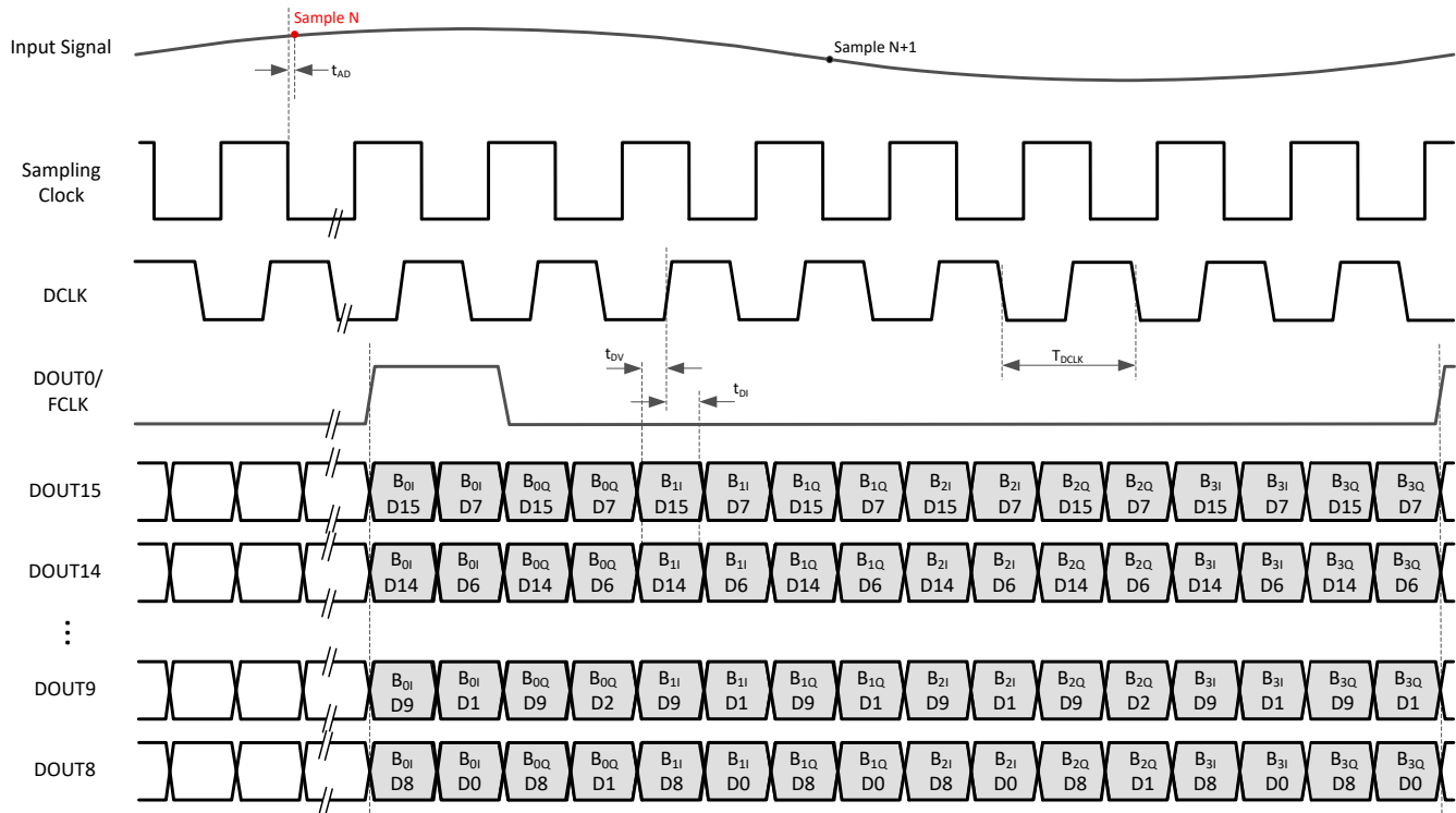
Figure 7-2. Timing Diagram: Serial LVDS (example: quad band, 16-bit, complex decimation by 8)
