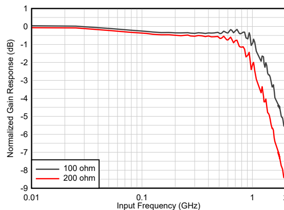
Figure 8-6. Full power input bandwidth for 100 and 200Ω internal termination
