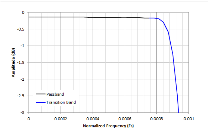
Figure 8-41. Decimation by 512 Passband Ripple Response
