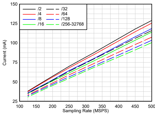
Figure 6-57. Current vs Sampling Rate Real Decimation, DVDD12
