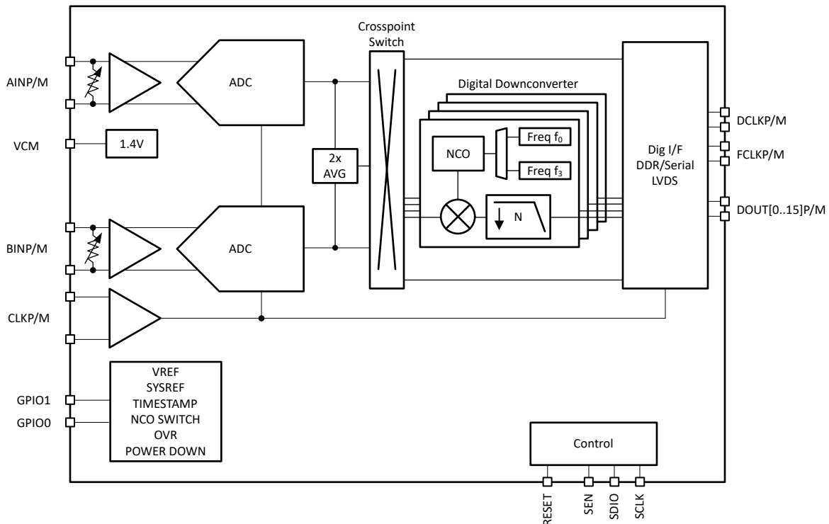
Figure 8-1. Block Diagram
