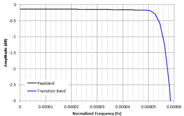
Figure 8-49. Decimation by 8192 Passband Ripple Response
