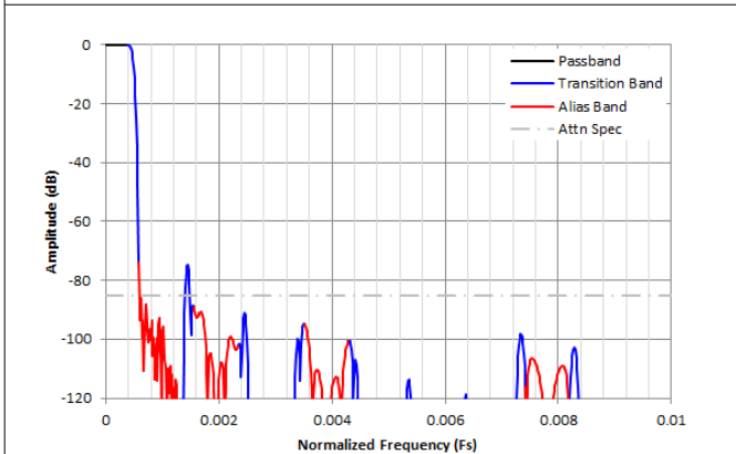
Figure 8-42. Complex Decimation by 1024 Filter Response
