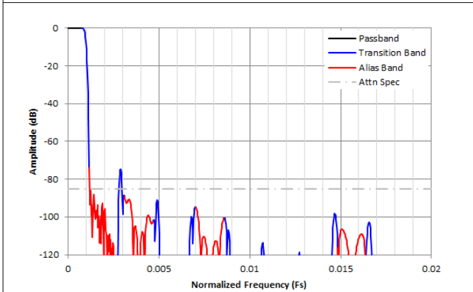
Figure 8-40. Complex Decimation by 512 Filter Response
