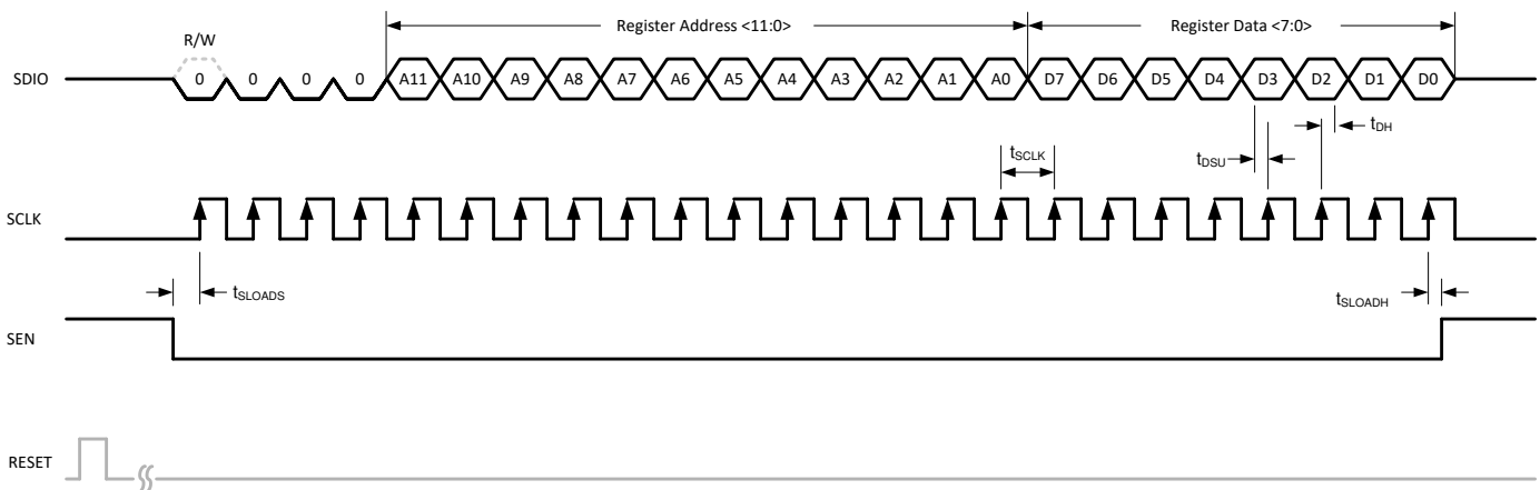
Figure 8-76. Serial Register Write Timing Diagram
