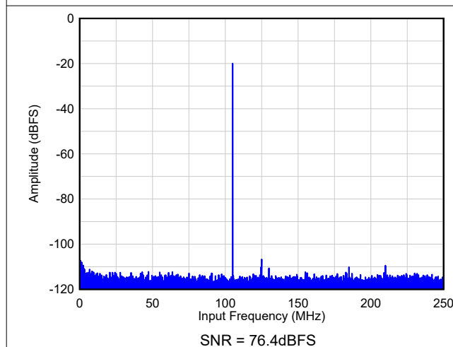
Figure 8-74. FFT - no AVG ( F_{IN} = 105\text{MHz} , A_{IN} = -20\text{dBFS} )
