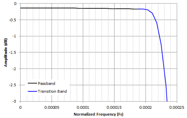
Figure 8-45. Decimation by 2048 Passband Ripple Response
