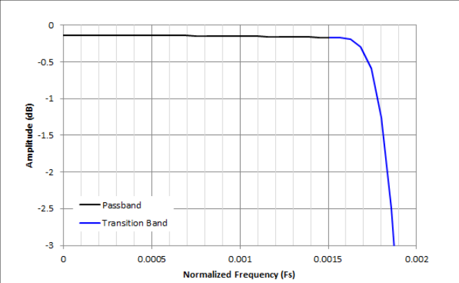
Figure 8-39. Decimation by 256 Passband Ripple Response
