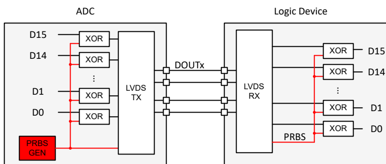
Figure 8-64. Output Scrambler
