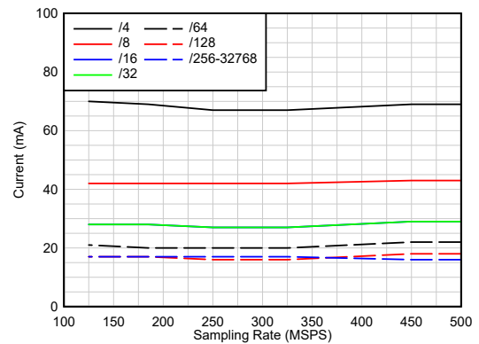
Figure 6-60. Current vs Sampling Rate Complex Decimation, Quad Band, DVDD18
