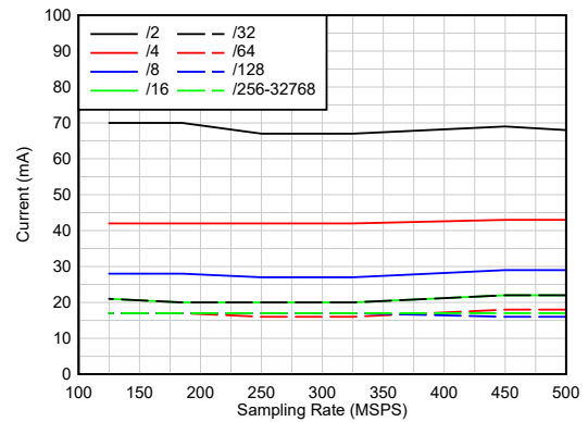
Figure 6-58. Current vs Sampling Rate Complex Decimation, Dual Band, DVDD18
