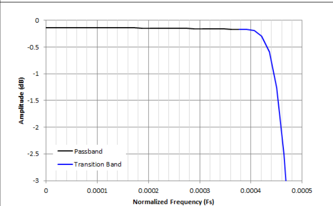
Figure 8-43. Decimation by 1024 Passband Ripple Response
