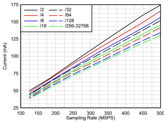
Figure 6-59. Current vs Sampling Rate Complex Decimation, Dual Band, DVDD12
