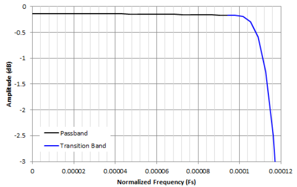
Figure 8-47. Decimation by 4096 Passband Ripple Response
