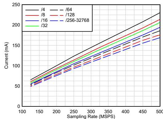
Figure 6-61. Current vs Sampling Rate Complex Decimation, Quad Band, DVDD12
