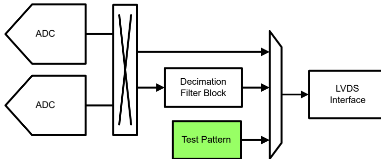
Figure 8-67. Test Pattern Generator
