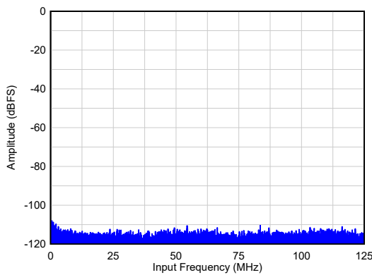
Figure 6-1. Idle Channel Noise
