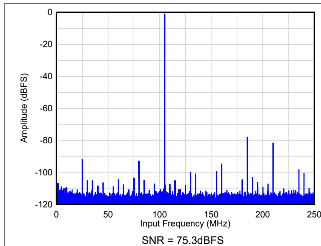
Figure 8-72. FFT - no AVG ( F_{IN} = 105\text{MHz} , A_{IN} = -1\text{dBFS} )
