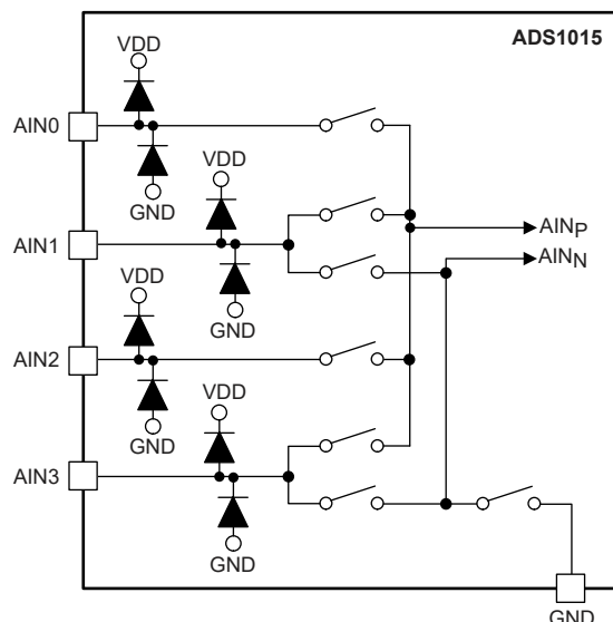
Figure 7-4. Input Multiplexer
