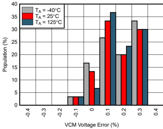
Figure 5-64. VCM Output Voltage Histogram
