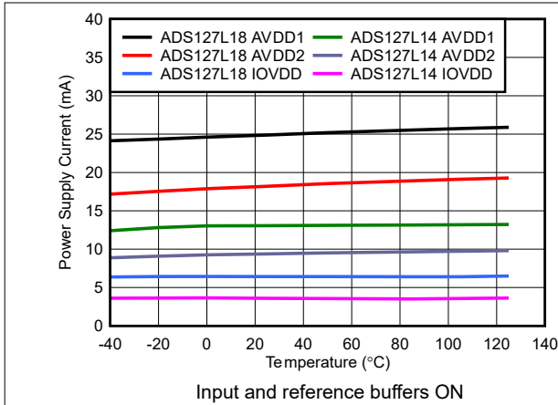
Figure 5-68. Mid-Speed Mode Power Supply Currents vs. Temperature
