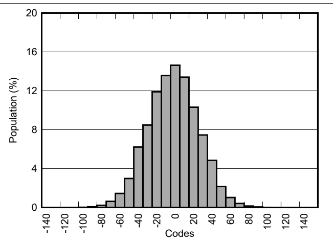
Figure 5-19. High-Speed Mode, Shorted Noise Histogram
