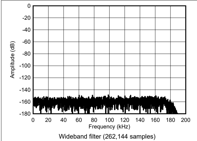
Figure 5-14. High-Speed Mode, Shorted FFT
