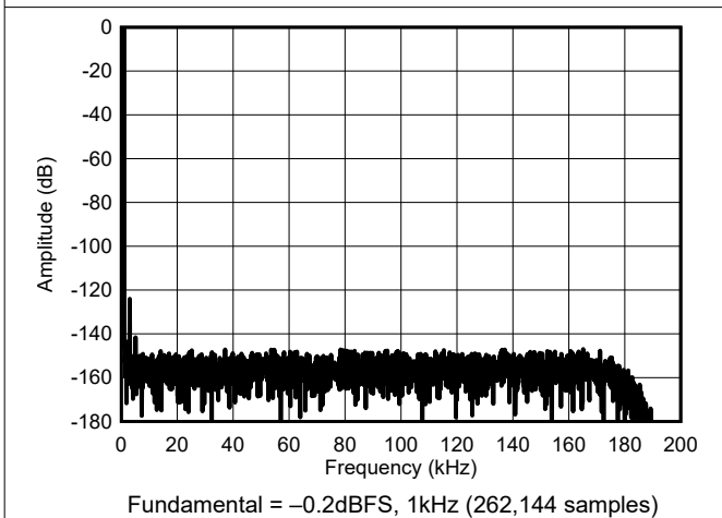
Figure 5-18. High-Speed Mode, Full-Scale FFT
