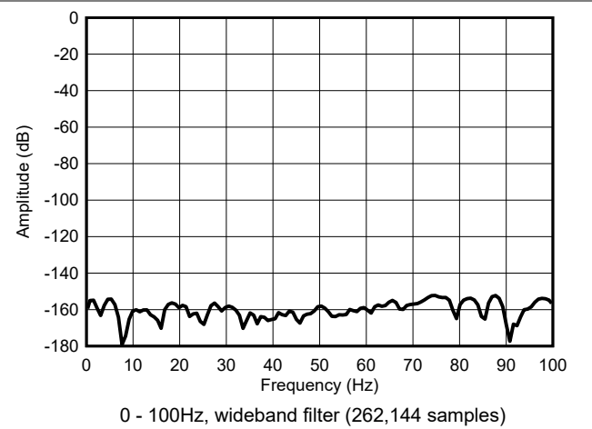
Figure 5-15. High-Speed Mode, Shorted FFT
