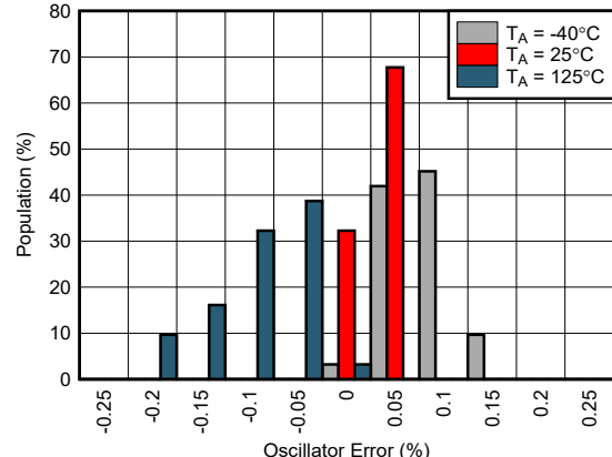
Figure 5-63. Oscillator Frequency Histogram
