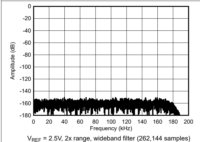
Figure 5-16. High-Speed Mode, Shorted FFT
