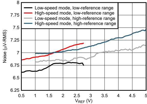
Wideband filter, OSR = 64 Figure 5-38. Integrated Noise vs. V REF
