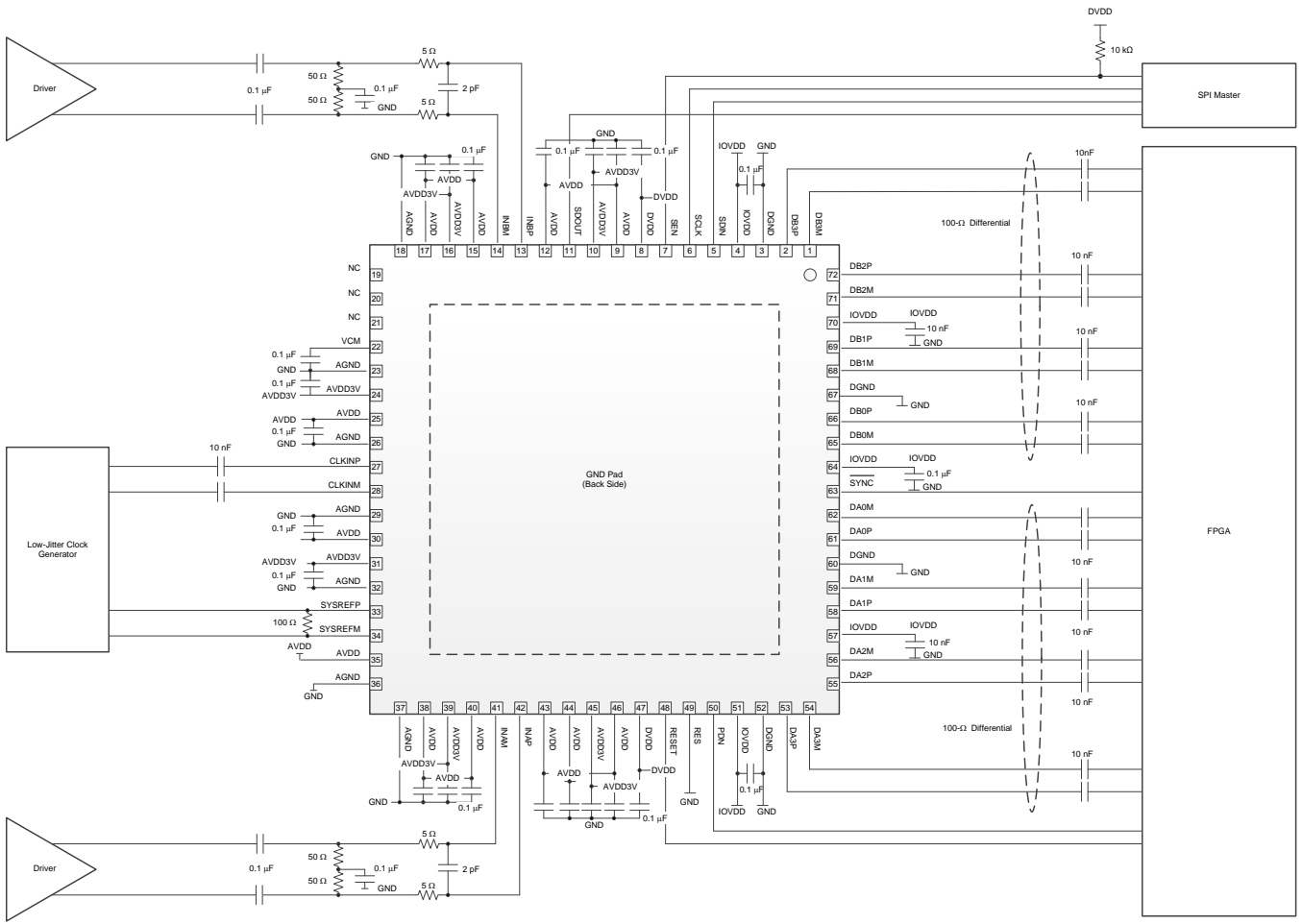
Figure 131. AC-Coupled Receiver
