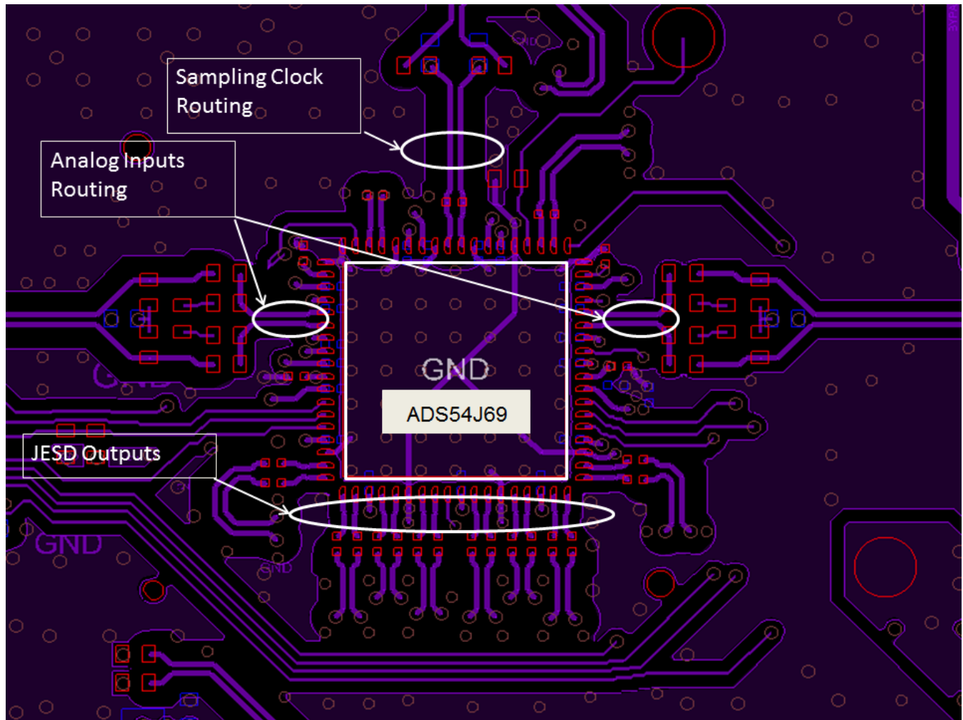
Figure 138. ADS54J69EVM layout
