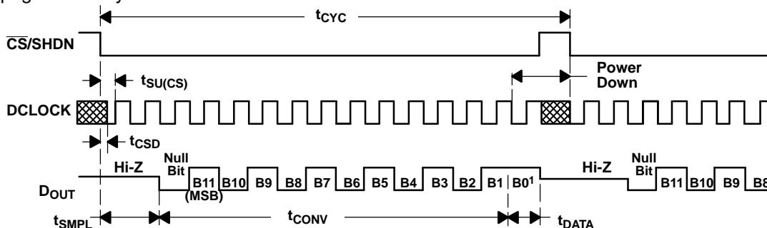
Figure 36. ADS7829 Timing
