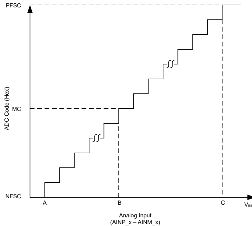
Figure 6-9. Transfer Characteristics
