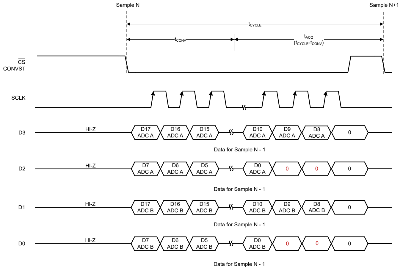
Figure 5-4. Conversion Cycle Timing: 4-Lane Mode with \overline{\text{CS}} and \text{CONVST} Shorted
