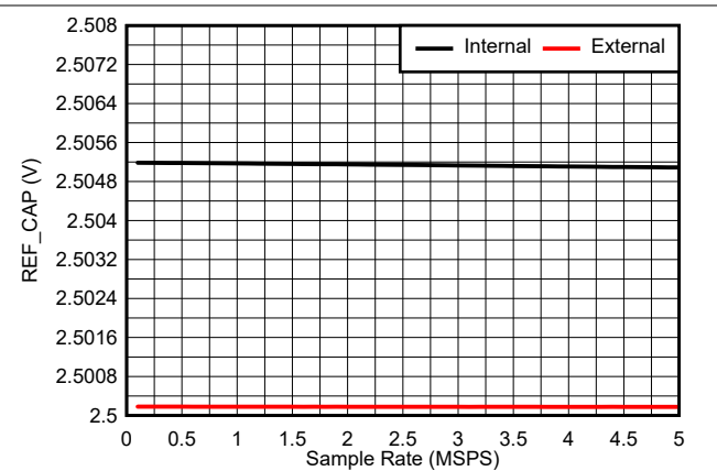
Figure 5-38. REF_CAP vs Sample Rate With 2.5V Reference
