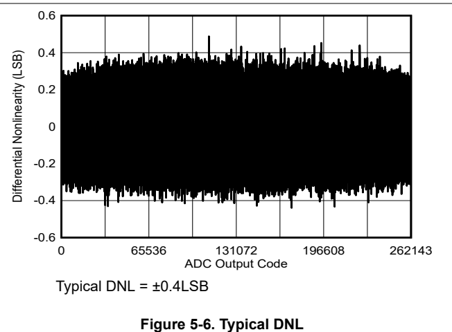
Figure 5-6. Typical DNL
