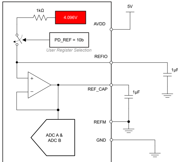
Figure 6-2. Internal Reference: AVDD = 5V
