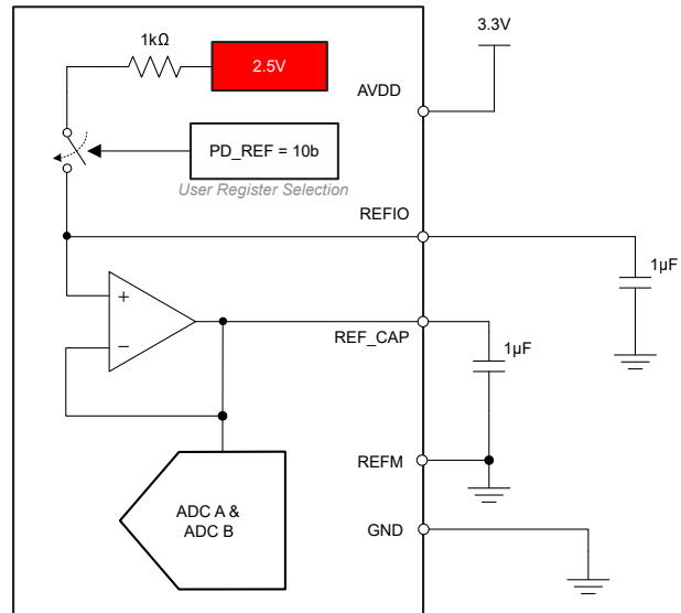
Figure 6-3. Internal Reference: AVDD = 3.3V
