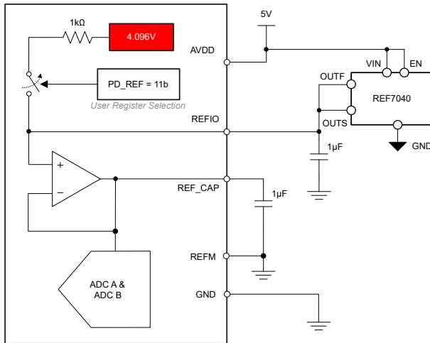
Figure 6-4. External Reference: AVDD = 5V
