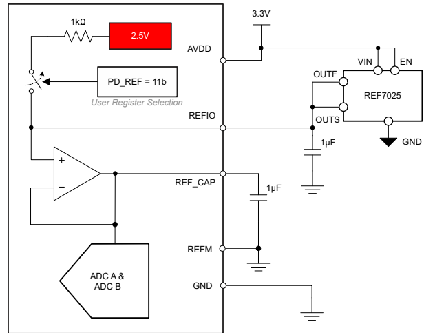
Figure 6-5. External Reference: AVDD = 3.3V
