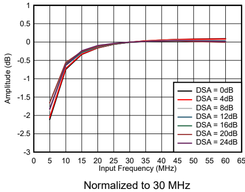
Figure 5-1. RX In-Band Gain Flatness, f_{IN} = 30\text{ MHz}
