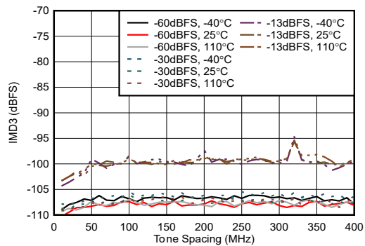
Figure 5-223. RX IMD3 vs Tone Spacing at 6.851 GHz
