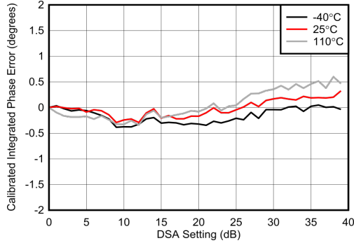
Figure 5-571. Calibrated Integrated Phase Error vs Temperature at 7.1 GHz
