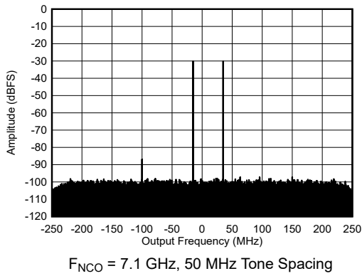
Figure 5-218. Dual Tone RX Output FFT at 7.1 GHz and -30 dBFS per Tone
