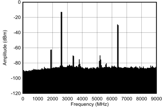
f_{\text{DAC}} = 9000 MSPS, external clock mode, non-interleave mode
