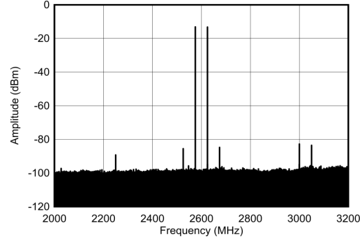
f_{\text{DAC}} = 9000 MSPS, external clock mode, non-interleave mode
