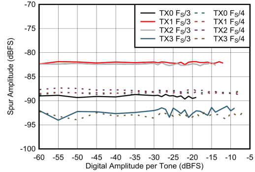
Figure 5-425. Two Tone Inband Fixed Spurs vs Digital Amplitude at 2.6 GHz
