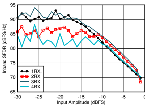
Figure 5-107. RX In-Band SFDR ( \pm 400\text{ MHz} ) vs Input Amplitude at 1.75 GHz
