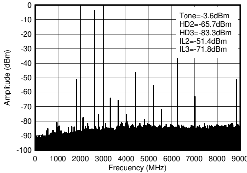
Figure 5-426. TX Single Tone (-12 dBFS) Output Spectrum at 2.6 GHz (0- f_{DAC} )
