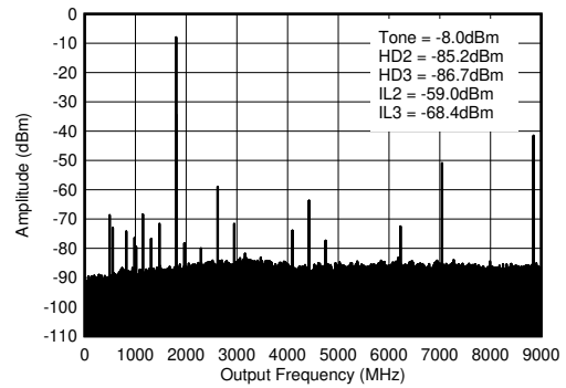
f_{\text{DAC}} = 8847.36 MSPS, interleave mode, 1.8 GHz matching, includes PCB and cable losses. \text{ILn} = f_{\text{S}}/n \pm f_{\text{OUT}} .
