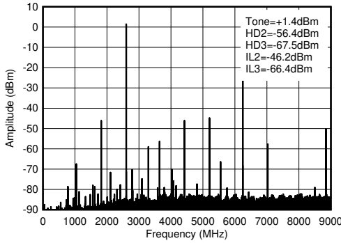
f_{\text{DAC}} = 8847.36 MSPS, interleave mode, 2.6 GHz matching, includes PCB and cable losses. \text{IL}_n = f_s/n \pm f_{\text{OUT}} .
