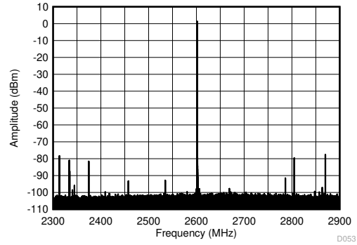
f_{\text{DAC}} = 8847.36 MSPS, interleave mode, 2.6 GHz matching, includes PCB and cable losses
