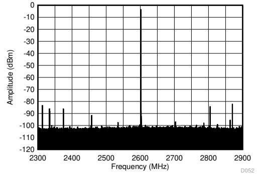
Figure 5-427. TX Single Tone (-12 dBFS) Output Spectrum at 2.6 GHz ( \pm 300 MHz)
