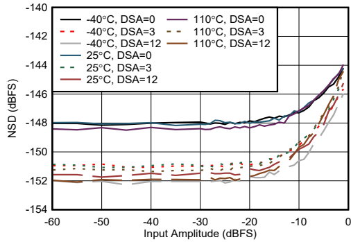
Figure 5-220. RX NSD vs Input Amplitude at 6.851 GHz
