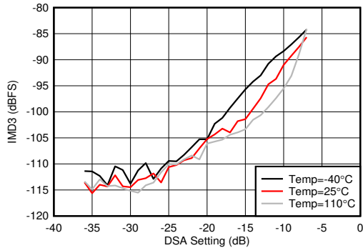
With 3.5 GHz matching, 20-MHz tone spacing
