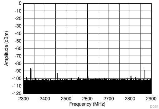
f_{\text{DAC}} = 8847.36 MSPS, straight mode, 2.6 GHz matching, includes PCB and cable losses
