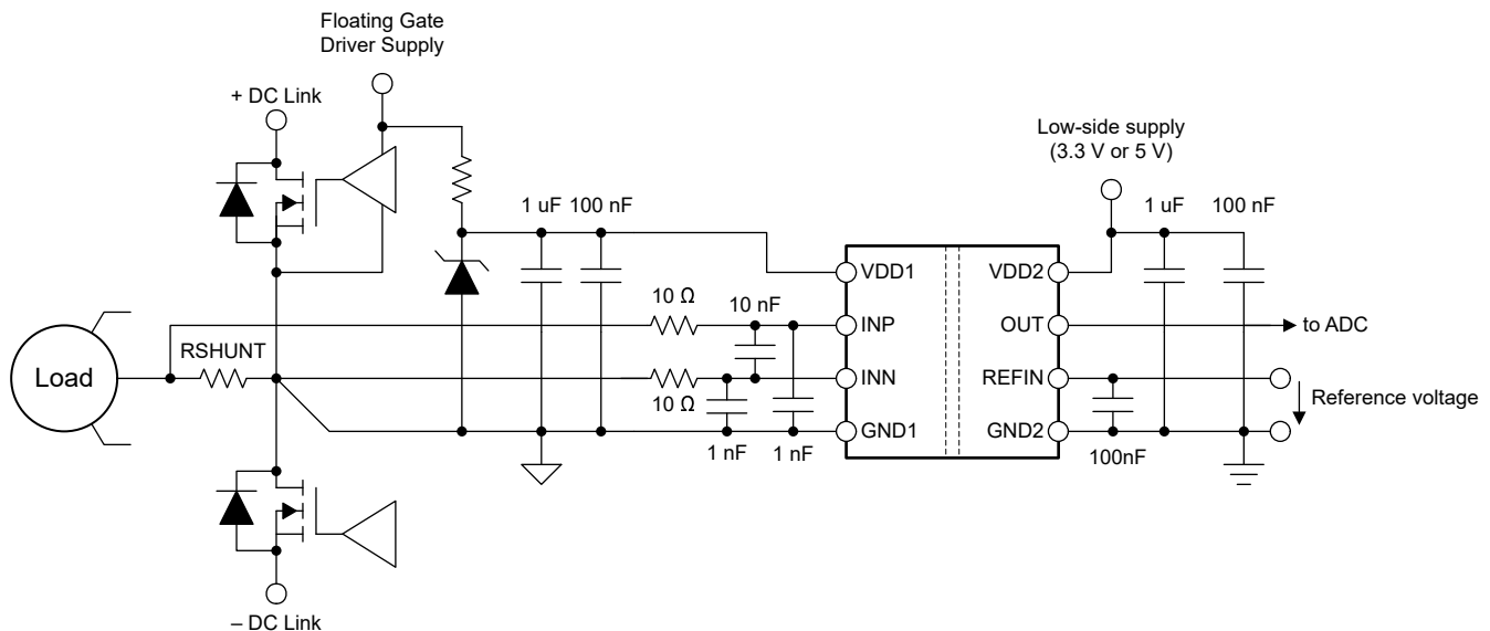
Figure 8-1. Using the AMC0x00R-Q1 for Current Sensing in a Typical Application
