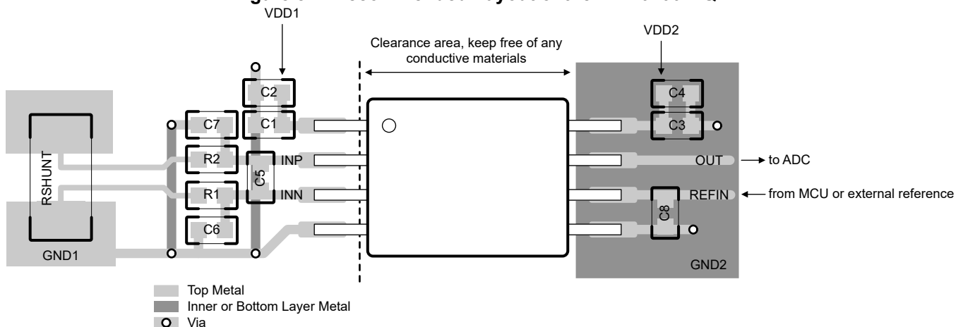
Figure 8-7. Recommended Layout of the AMC0x00R-Q1
