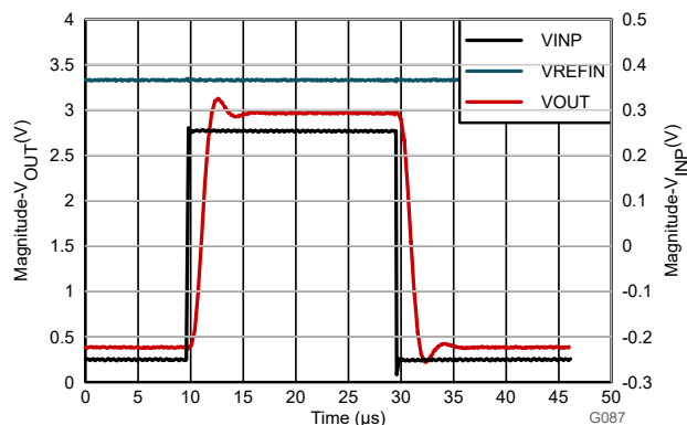
Figure 8-4. Output Step Response of the AMC0x00R-Q1
