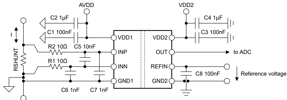
Figure 8-6. Decoupling of the AMC0x00R-Q1
