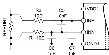
Figure 8-2. Input Filter
