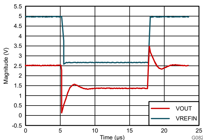
Figure 8-5. Reference Input Step Response of the AMC0x00R-Q1
