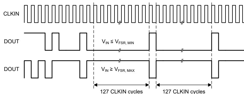
Figure 7-6. Full-Scale Output of the AMC0x06M05-Q1
