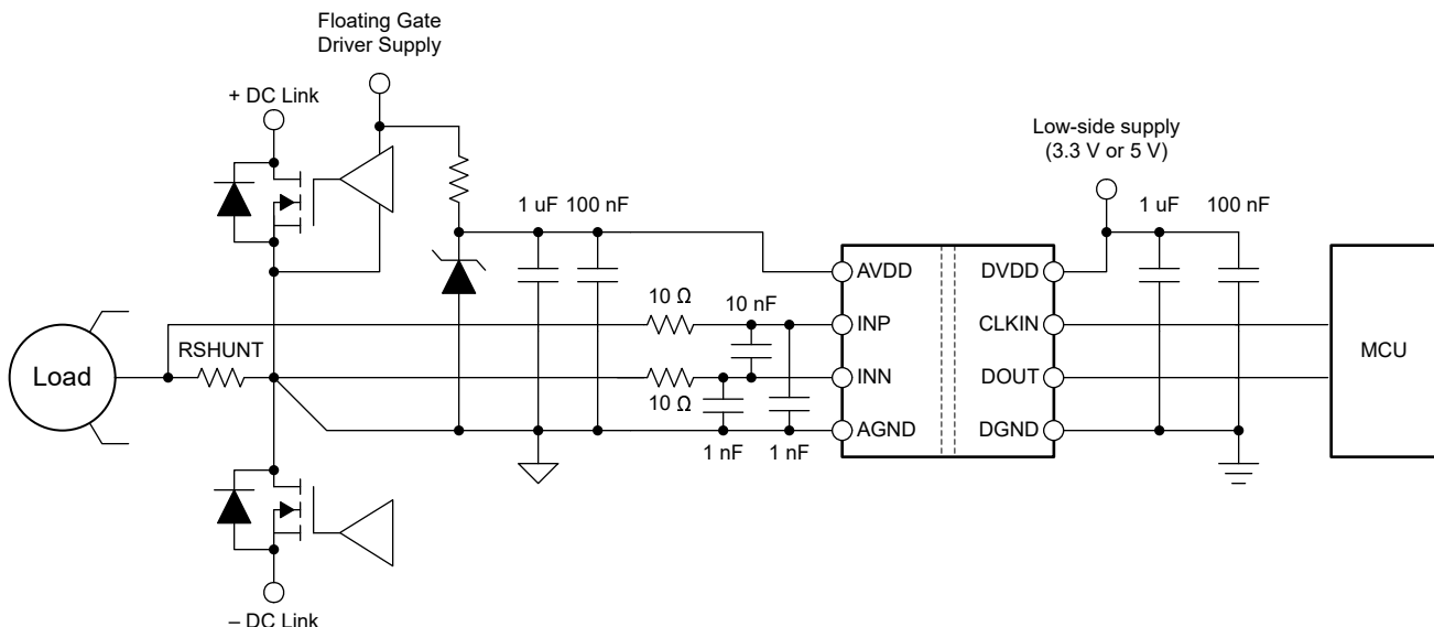
Figure 8-1. Using the AMC0x06M05-Q1 for Current Sensing in a Typical Application
