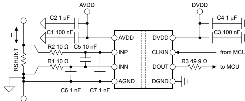
Figure 8-4. Decoupling of the AMC0x06M05-Q1
