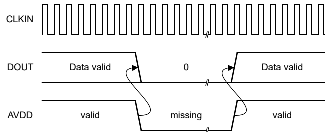
Figure 7-7. Output of the AMC0x06M05-Q1 in Case of a Missing High-Side Supply
