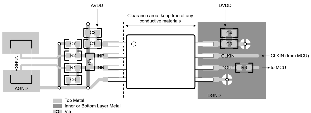
Figure 8-5. Recommended Layout of the AMC0x06M05-Q1
