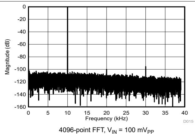
Figure 6-35. Frequency Spectrum With 10-kHz Input Signal
