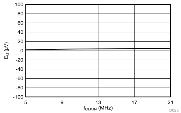
Figure 6-13. Offset Error vs Clock Frequency
