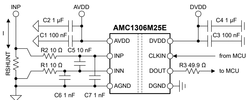
Figure 8-4. Decoupling of the AMC1306M25E
