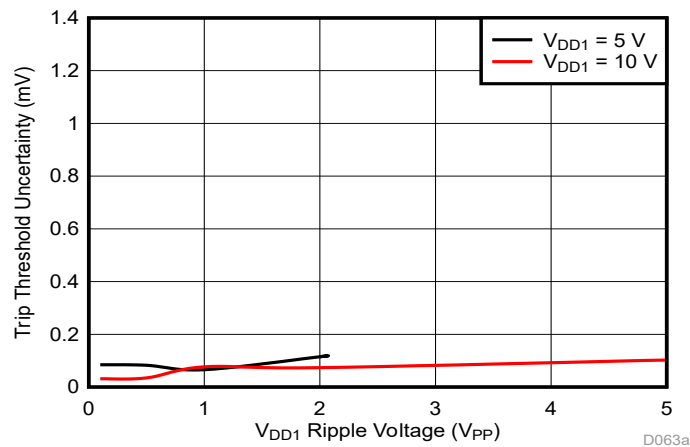
Figure 7-3. Trip Threshold Sensitivity to VDD1 Ripple Voltage (f RIPPLE = 10kHz)
