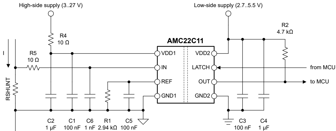
Figure 7-4. Decoupling of the AMC22C11
