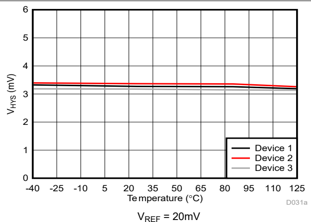
Figure 5-29. Cmp1 Trip Threshold Hysteresis vs Temperature
