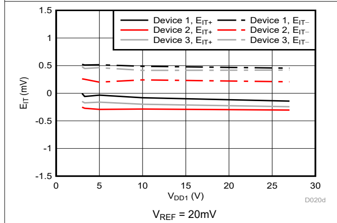
Figure 5-8. Cmp0 Trip Threshold Error vs Supply Voltage
