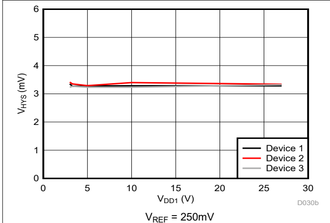
Figure 5-34. Cmp1 Trip Threshold Hysteresis vs Supply Voltage
