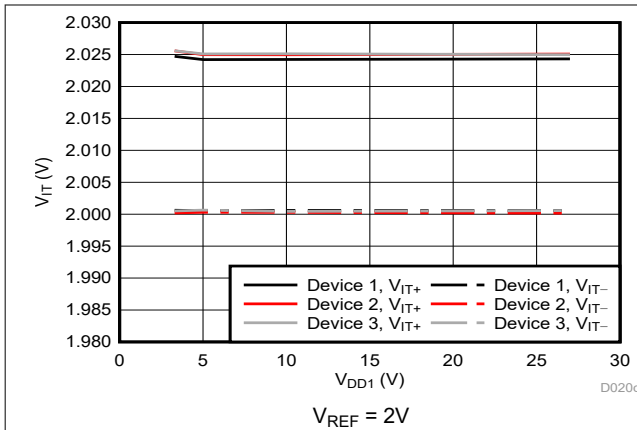
Figure 5-18. Cmp0 Trip Threshold vs Supply Voltage
