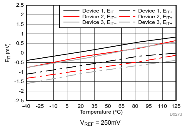
Figure 5-33. Cmp1 Trip Threshold Error vs Temperature
