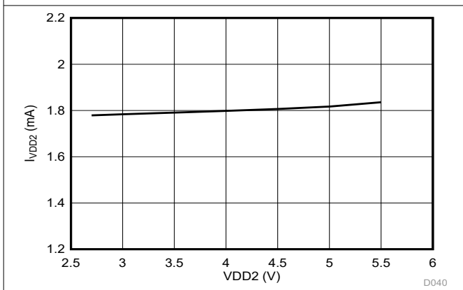
Figure 5-44. High-Side Supply Current vs Supply Voltage
