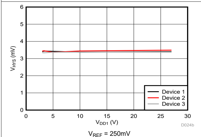
Figure 5-16. Cmp0 Trip Threshold Hysteresis vs Supply Voltage
