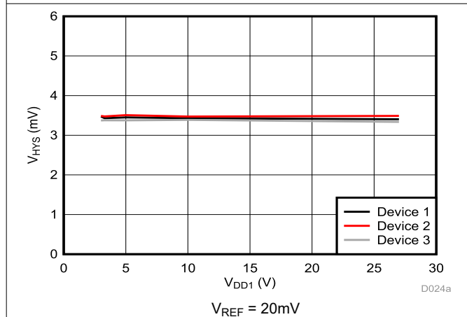
Figure 5-10. Cmp0 Trip Threshold Hysteresis vs Supply Voltage
