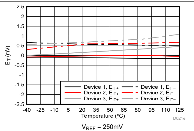
Figure 5-15. Cmp0 Trip Threshold Error vs Temperature
