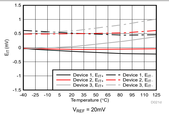
Figure 5-9. Cmp0 Trip Threshold Error vs Temperature
