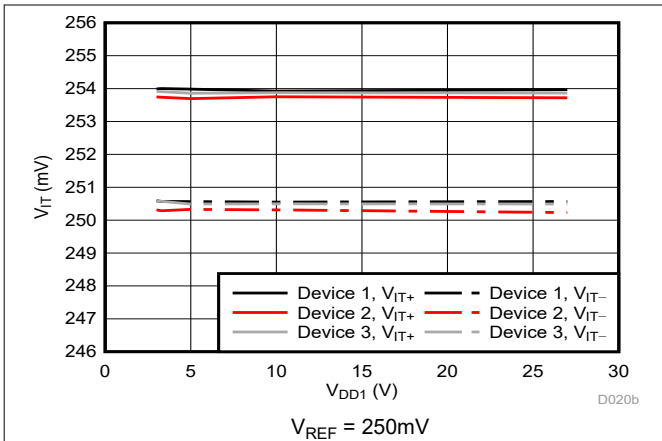
Figure 5-12. Cmp0 Trip Threshold vs Supply Voltage
