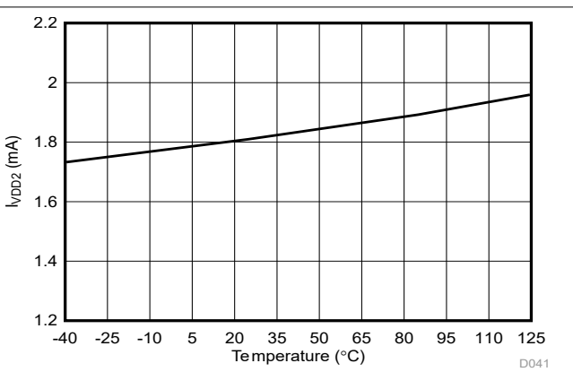
Figure 5-45. High-Side Supply Current vs Temperature
