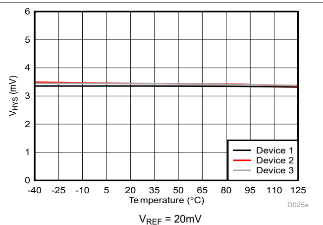
Figure 5-11. Cmp0 Trip Threshold Hysteresis vs Temperature
