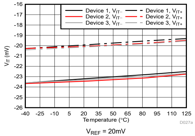
Figure 5-25. Cmp1 Trip Threshold vs Temperature
