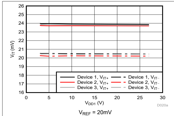
Figure 5-6. Cmp0 Trip Threshold vs Supply Voltage
