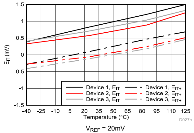
Figure 5-27. Cmp1 Trip Threshold Error vs Temperature
