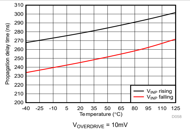
Figure 5-39. Cmp1 Propagation Delay vs Temperature
