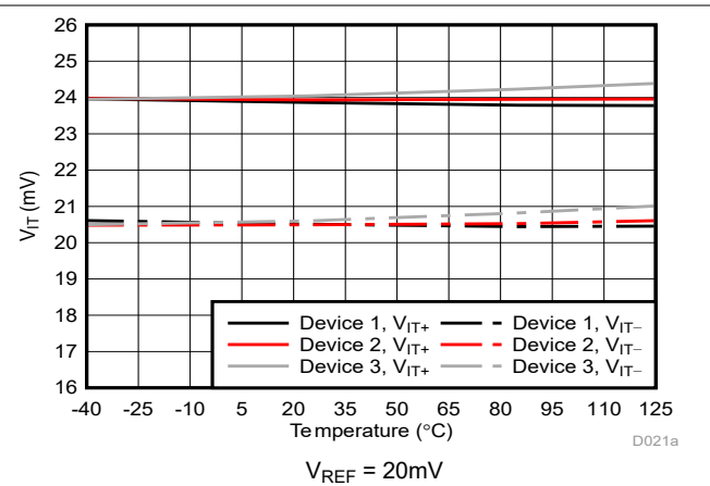
Figure 5-7. Cmp0 Trip Threshold vs Temperature
