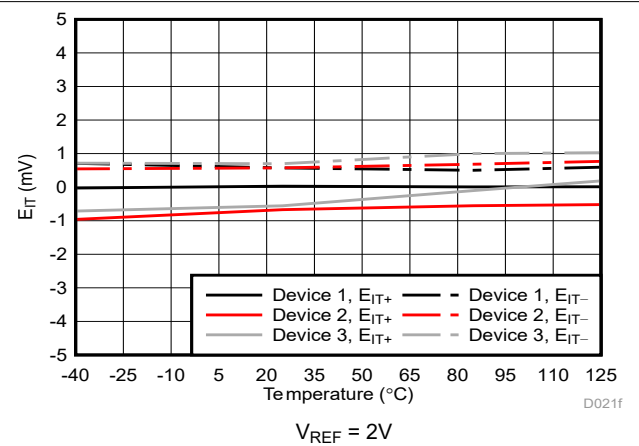
Figure 5-21. Cmp0 Trip Threshold Error vs Temperature
