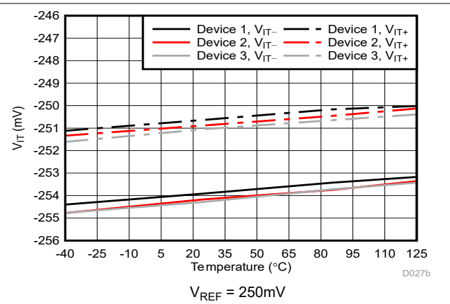
Figure 5-31. Cmp1 Trip Threshold vs Temperature
