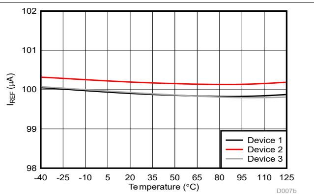
Figure 5-43. Reference Current vs Temperature
