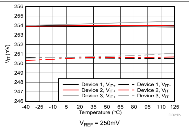
Figure 5-13. Cmp0 Trip Threshold vs Temperature
