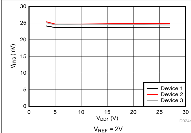
Figure 5-22. Cmp0 Trip Threshold Hysteresis vs Supply Voltage
