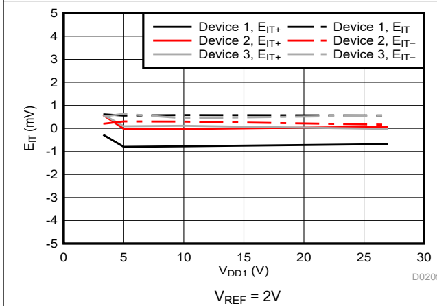
Figure 5-20. Cmp0 Trip Threshold Error vs Supply Voltage
