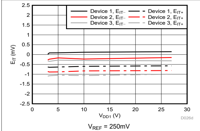
Figure 5-32. Cmp1 Trip Threshold Error vs Supply Voltage
