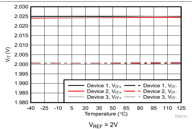
Figure 5-19. Cmp0 Trip Threshold vs Temperature
