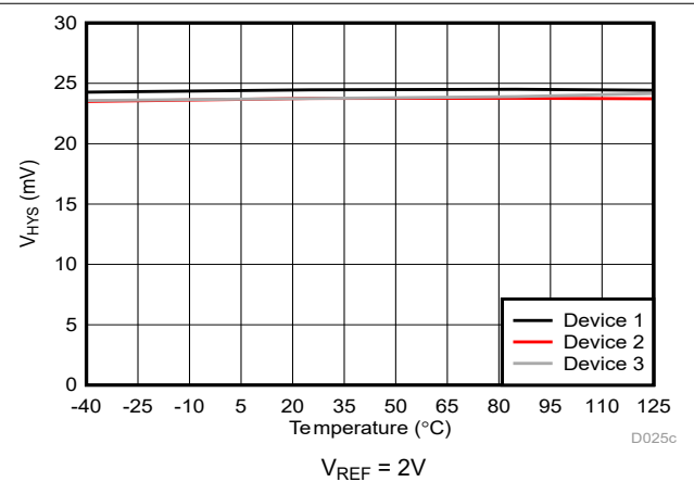
Figure 5-23. Cmp0 Trip Threshold Hysteresis vs Temperature
