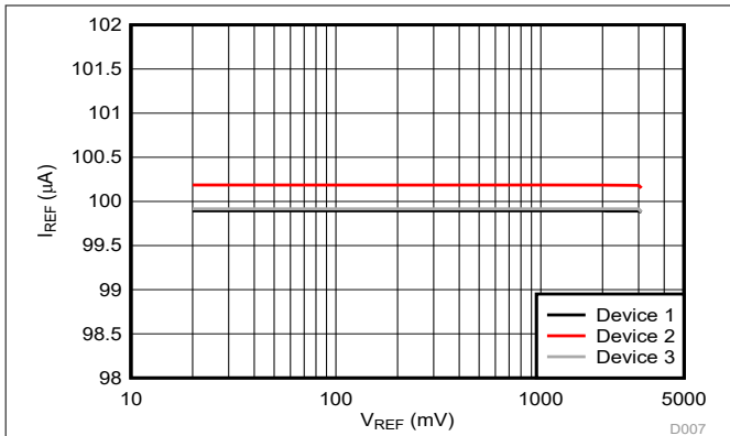
Figure 5-42. Reference Current vs Reference Voltage
