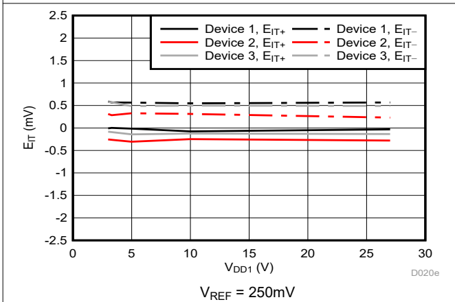
Figure 5-14. Cmp0 Trip Threshold Error vs Supply Voltage
