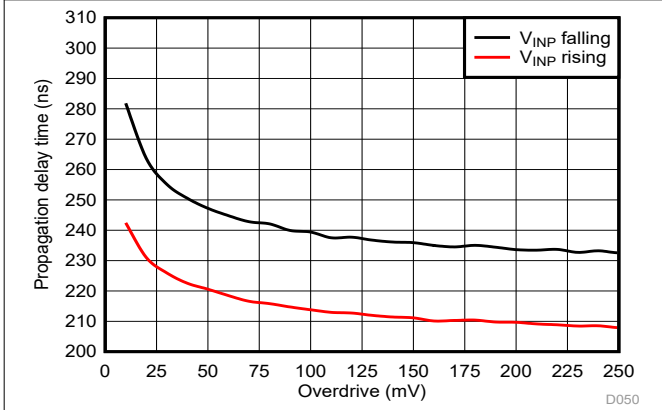
Figure 5-36. Cmp0 Propagation Delay vs Overdrive
