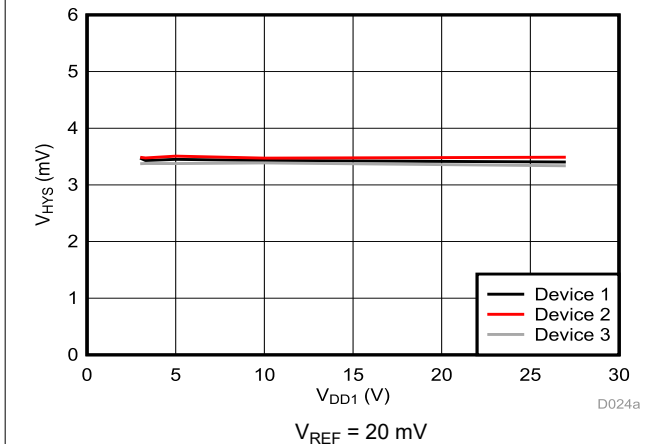
Figure 6-9. Cmp0 Trip Threshold Hysteresis vs Supply Voltage
