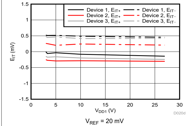
Figure 6-7. Cmp0 Trip Threshold Error vs Supply Voltage
