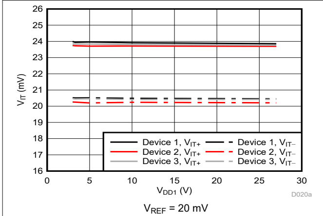
Figure 6-5. Cmp0 Trip Threshold vs Supply Voltage
