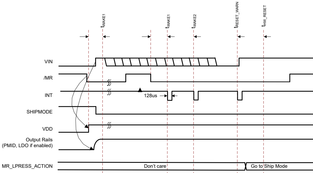
Figure 9-4. MR Wake from Ship Mode – VIN Dependencies
