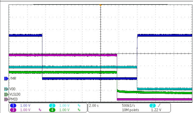
Figure 10-5. Power Up from Ship Mode with \overline{MR} Press
