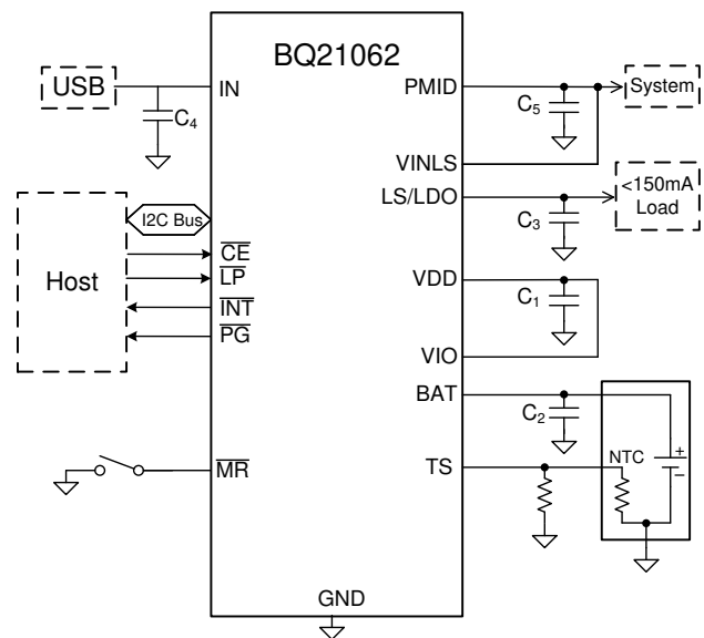
Simplified Schematic
