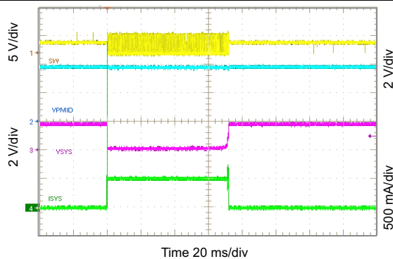
Figure 78. 3.3 V_{SYS} Load Transient, 0 to 200 mA
