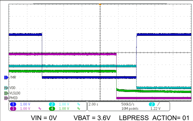
Figure 10-7. Ship Mode Entry with MR Long Button Press
