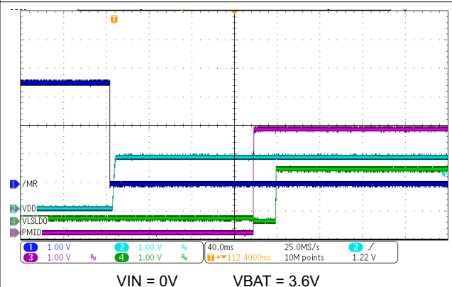
Figure 10-5. Power Up from Ship Mode with MR Press
