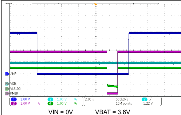
Figure 10-6. HW Reset on MR Long Button Press
