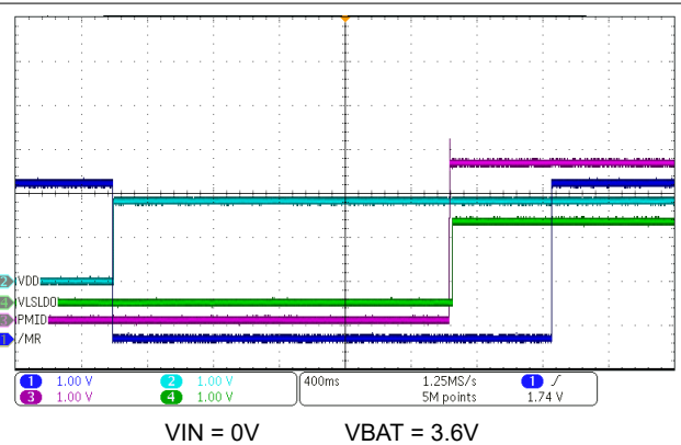
Figure 10-5. Power Up from Ship Mode with \overline{MR} Press
