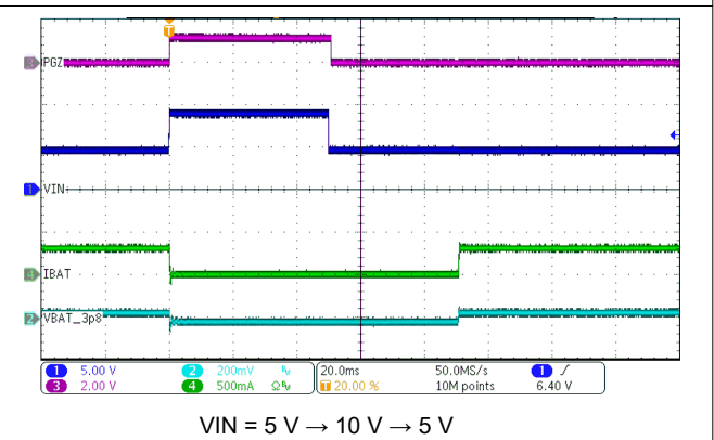
Figure 8-7. IN OVP Response
