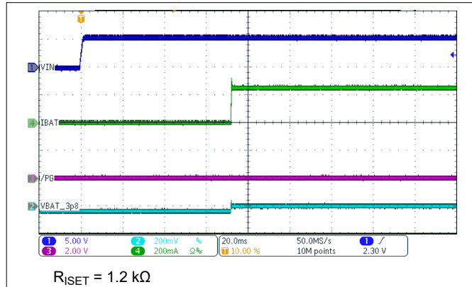
Figure 8-2. Power Up With Battery
