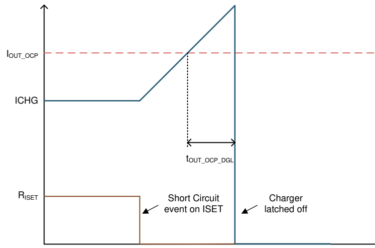
Figure 7-4. Overcurrent Protection
