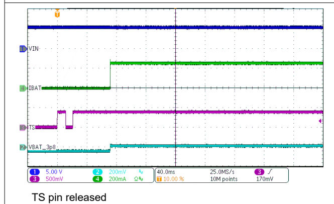
Figure 8-6. Charge Enable
