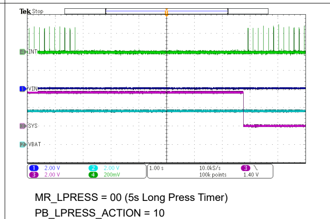
Figure 7-7. Enter Shipmode with Push Button Long Press
