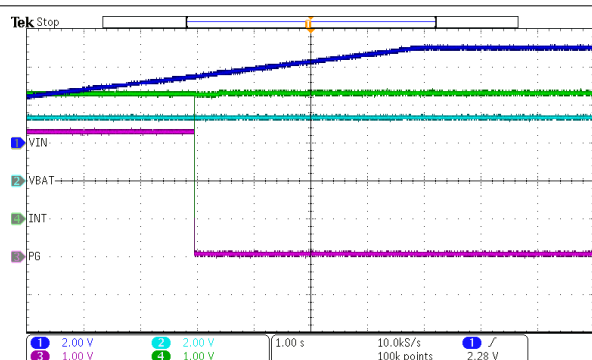
Figure 7-16. Wake2 Interrupt with VIN Present
