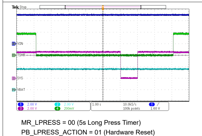
Figure 7-6. Hardware Reset with /TSMR Press
