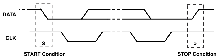
Figure 6-9. START and STOP Condition
