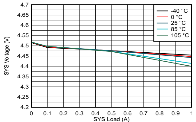
Figure 5-4. SYS Load Regulation
