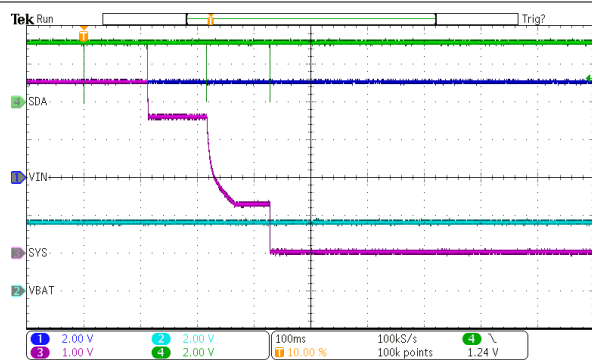
Figure 7-14. SYS Mode Sweep
