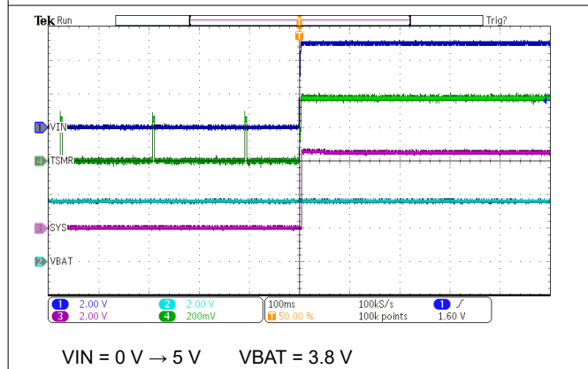
Figure 7-4. Power Up from Shipmode with VIN Insertion
