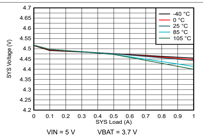
Figure 5-4. SYS Load Regulation
