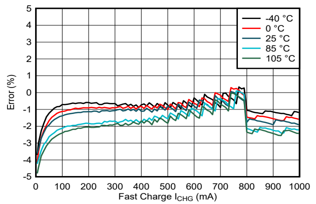
Figure 5-2. Charge Current Accuracy vs ICHARGE Setting
