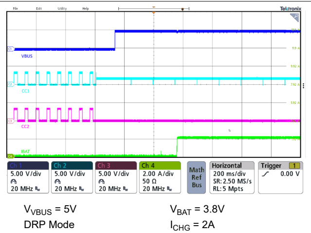
Figure 8-3. USB-C Adapter Plug-In, DRP Mode
