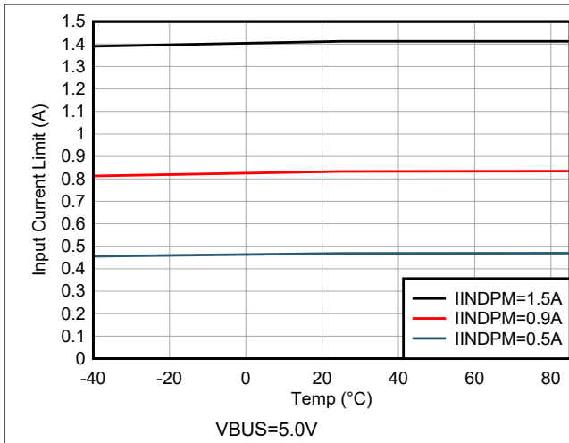
Figure 6-9. Input Current Regulation vs Temperature
