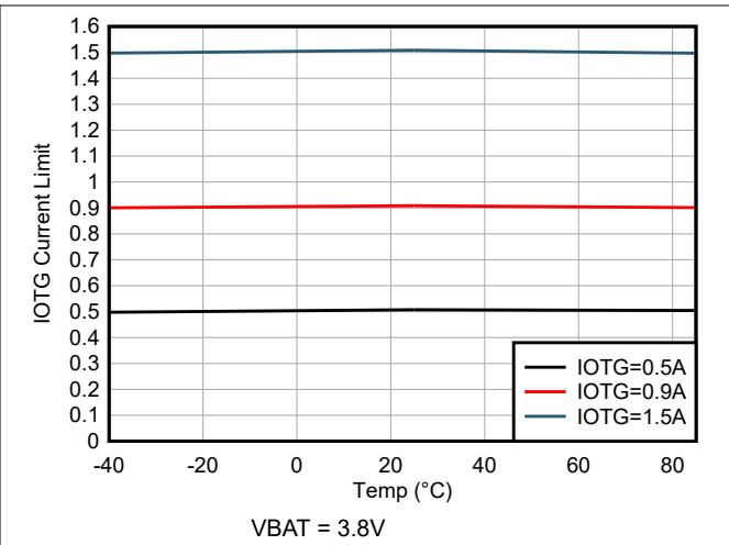
Figure 6-10. OTG Mode Current Regulation vs Temperature
