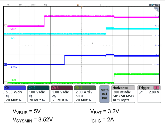
Figure 8-5. Power-Up Sequence
