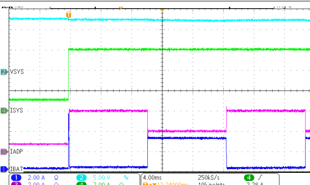
Figure 8-22. Automatic Second Phase Adding and Dropping Under 28-V VBUS
