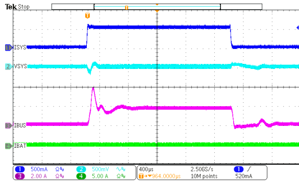
Figure 8-13. System Regulation in Boost Mode
