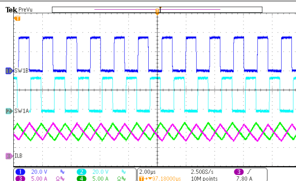
Figure 8-20. Dual Phase Current Balance at 36 V 180 W
