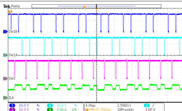
Figure 8-8. PWM Operation
