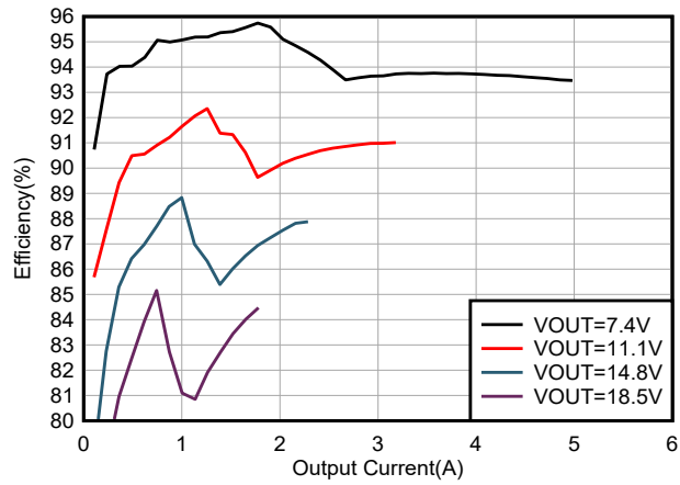
Figure 6-1. System Efficiency
