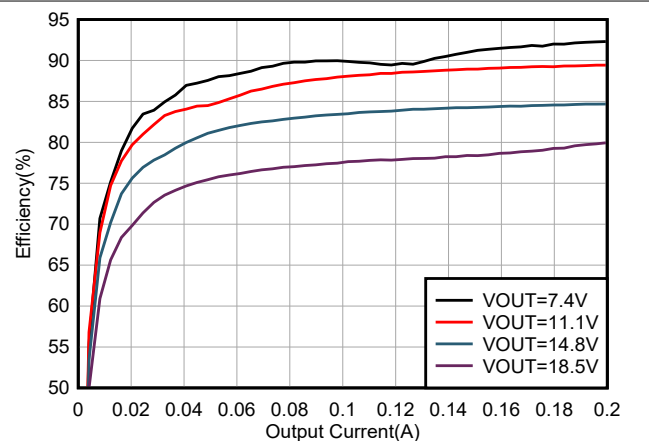
Figure 6-4. System Efficiency
