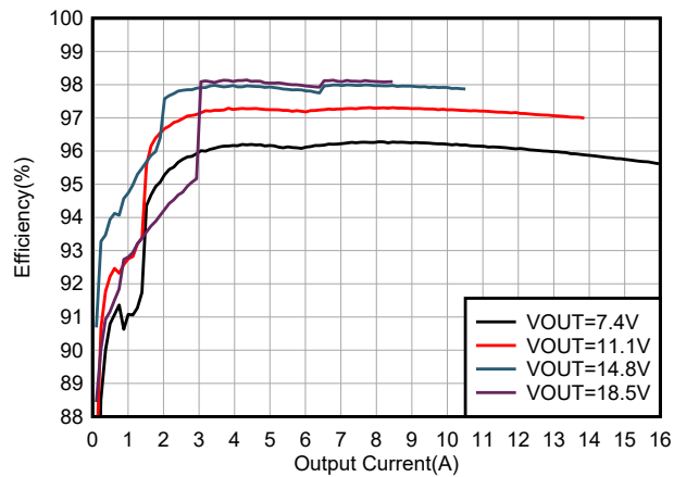
Figure 6-1. System Efficiency
