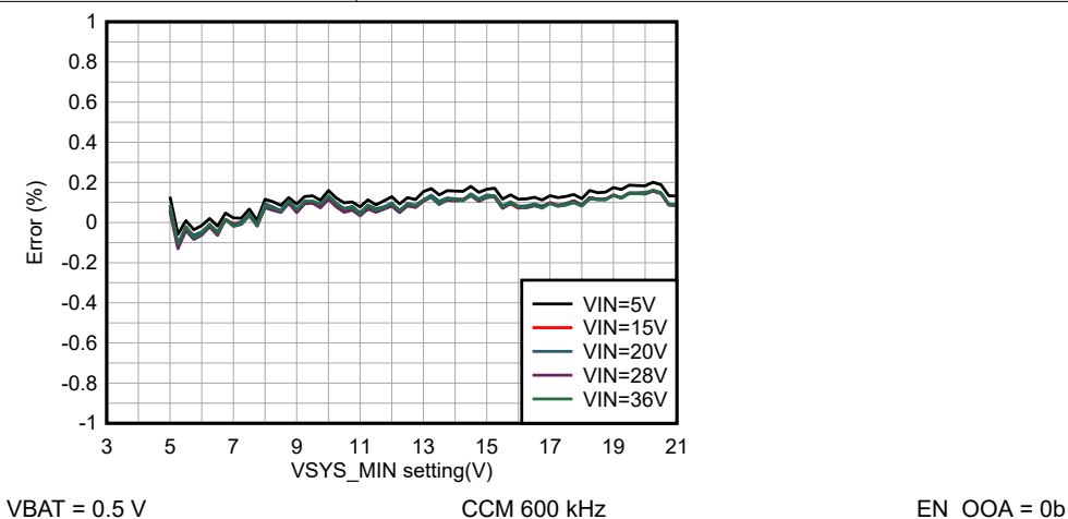
Figure 6-17. Minimum System Voltage Regulation Accuracy
