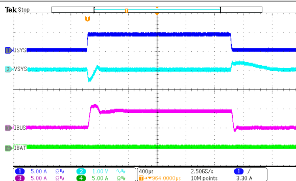
Figure 8-10. Switching During Buck Boost Mode
