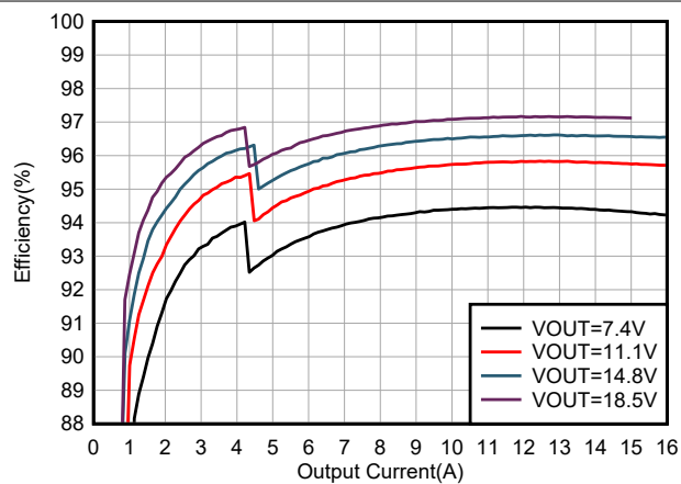
Figure 6-3. System Efficiency
