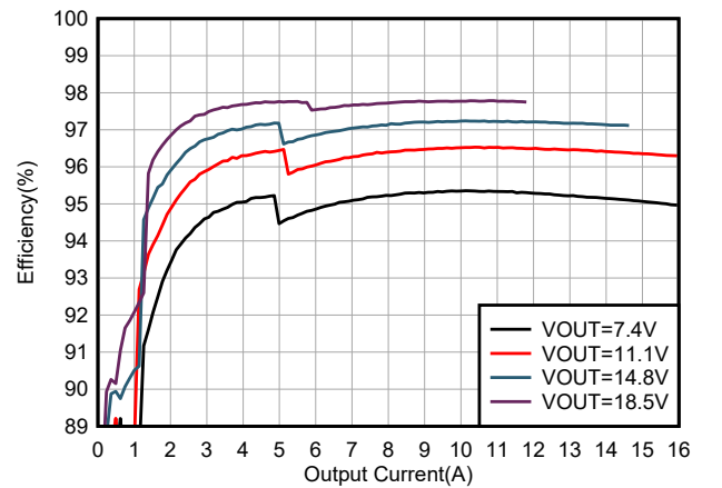
Figure 6-2. System Efficiency
