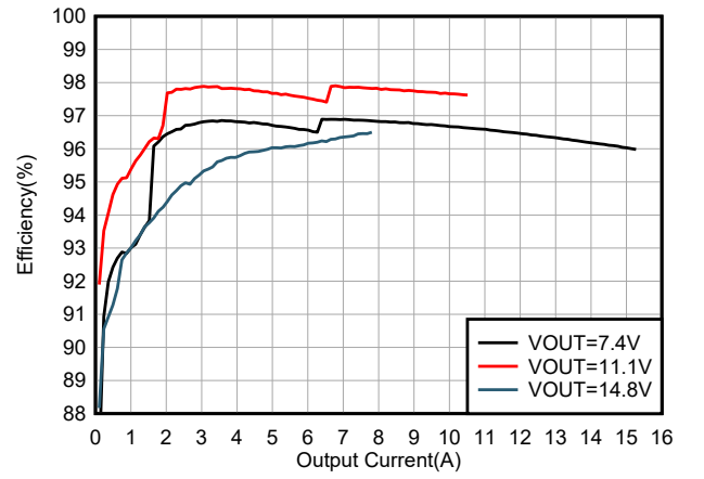
Figure 6-2. System Efficiency
