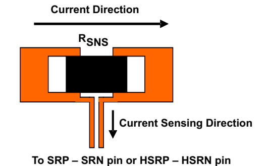
Figure 45. Sensing Resistor PCB Layout
