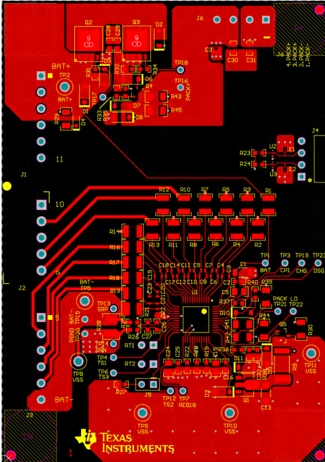
Figure 8-10. BQ76952 Two-Layer Board Layout–Top Layer
