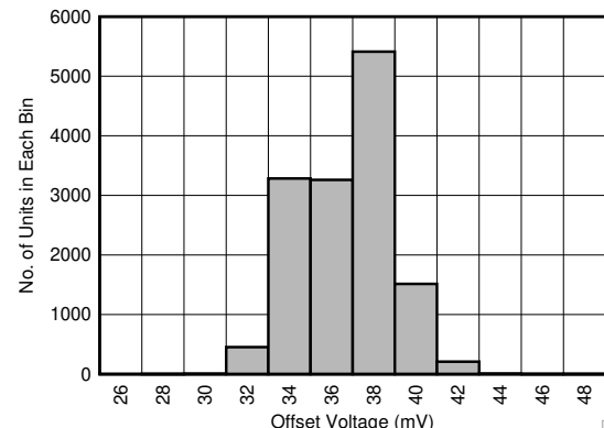
14000 devices, \mu = 35.7\text{ mV} , \sigma = 2.15\text{ mV} Figure 6-42. Offset Voltage Distribution Histogram
