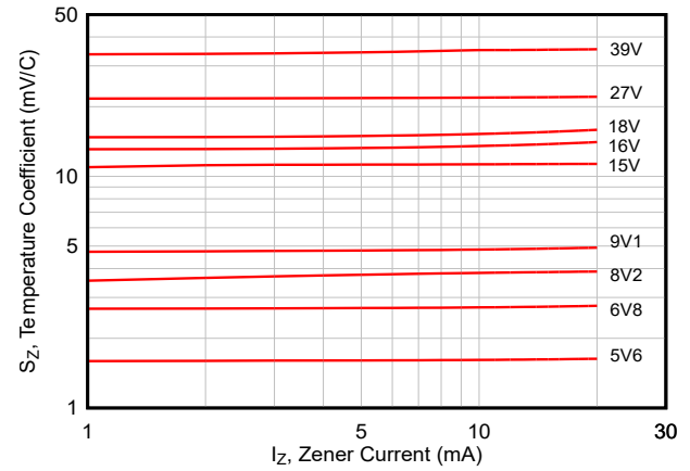
Figure 5-2. Temperature Coefficient
