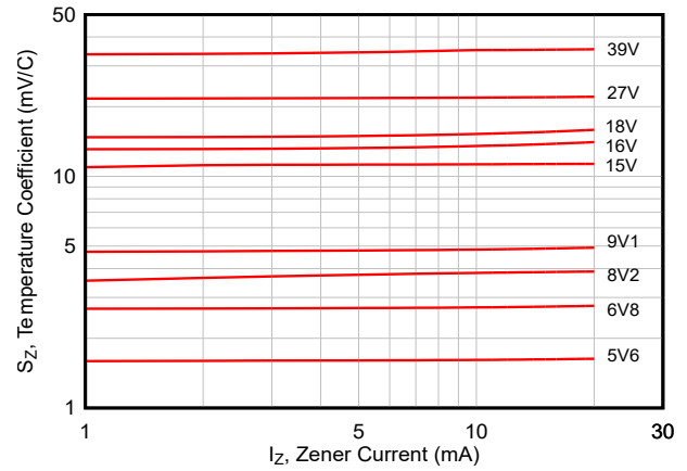
Figure 5-2. Temperature Coefficient
