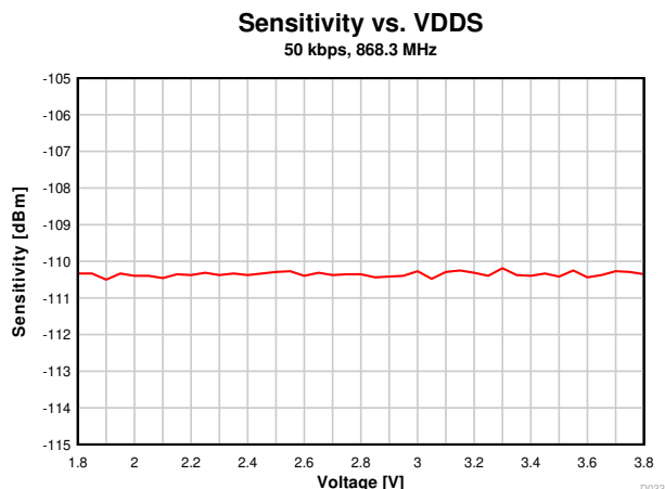
Figure 7-16. Sensitivity vs Supply Voltage (VDD) (50kbps, 868.3MHz)
