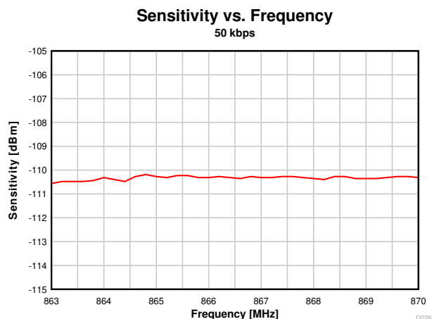
Figure 7-13. Sensitivity vs Frequency (50kbps, 868MHz)
