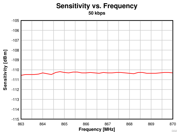
Figure 7-11. Sensitivity vs Frequency (50kbps, 868MHz)
