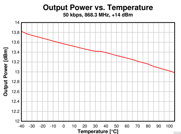
Figure 7-19. Output Power vs Temperature (50kbps, 868.3MHz)
