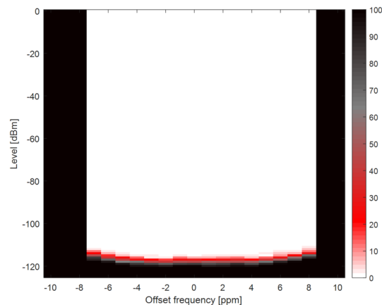
Figure 7-18. Narrowband, 9.6kbps \pm 2.4 kHz Deviation, 2-GFSK, 868MHz, 17.1kHz RX Bandwidth
