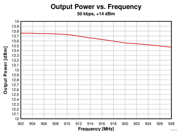
Figure 7-22. Output Power vs Frequency (50kbps, 915MHz)
