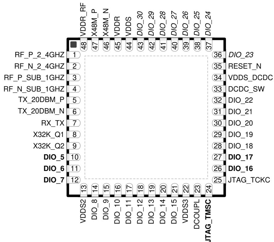
Figure 6-1. RGZ (7-mm x 7-mm) Pinout, 0.5-mm Pitch (Top View)
