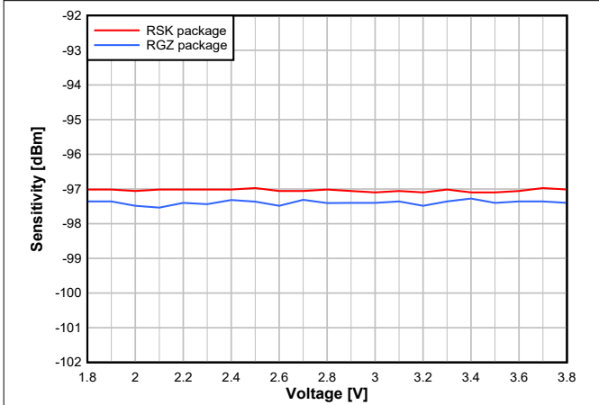
Figure 8-22. Sensitivity vs. Supply Voltage (VDD5) (BLE 1 Mbps, 2.44 GHz)
