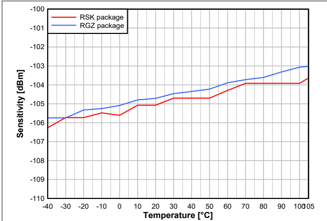
Figure 8-20. Sensitivity vs. Temperature (250 kbps, 2.44 GHz)
