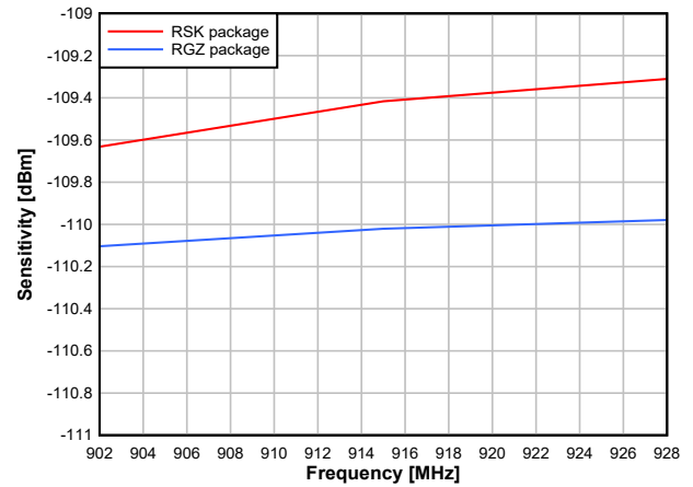
Figure 8-15. Sensitivity vs. Frequency (50 kbps, 915 MHz)
