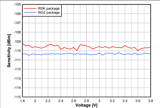
Figure 8-21. Sensitivity vs. Supply Voltage (VDD5) (50 kbps, 868.3 MHz)
