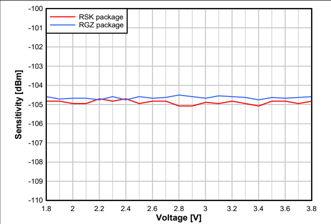
Figure 8-23. Sensitivity vs. Supply Voltage (VDD5) (250 kbps, 2.44 GHz)
