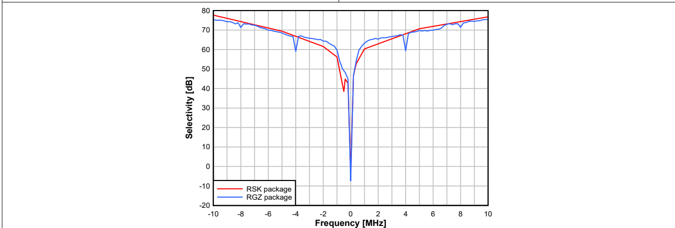
Figure 8-24. Selectivity vs. Frequency Offset (50 kbps, 868.3 MHz)
