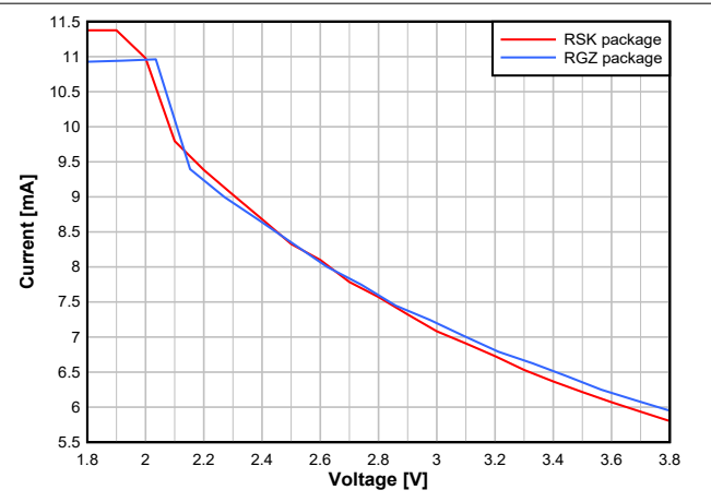
Figure 8-13. TX Current vs. Supply Voltage (VDD) (BLE 1 Mbps, 2.44 GHz, 0 dBm)
