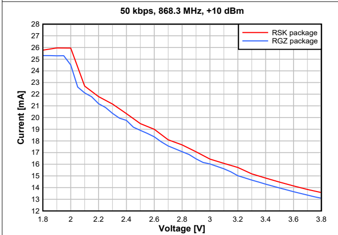
Figure 8-12. TX Current vs. Supply Voltage (VDD) (50 kbps, 868.3 MHz)
