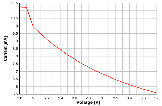
Figure 8-7. RX Current vs. Supply Voltage (VDDS) (BLE 1 Mbps, 2.44 GHz)
