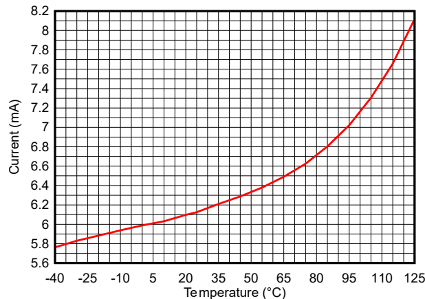
Figure 7-8. RX Current vs Temperature (BLE 1Mbps, 2.44GHz), V_{DD} = 3.3\text{V}
