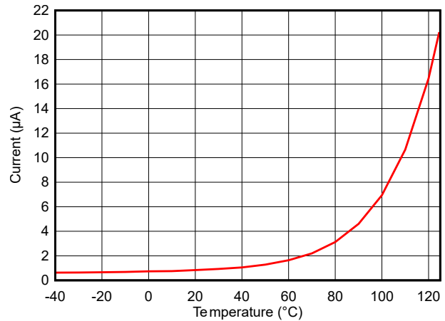
Figure 7-7. Standby Mode (MCU) Current vs Temperature (SRAM and partial register retention, RTC enabled), V_{DD} = 3.3\text{V}
