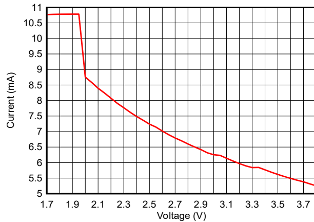
Figure 7-6. Active Mode (MCU) Current vs Supply Voltage (VDD) (Running CoreMark)
