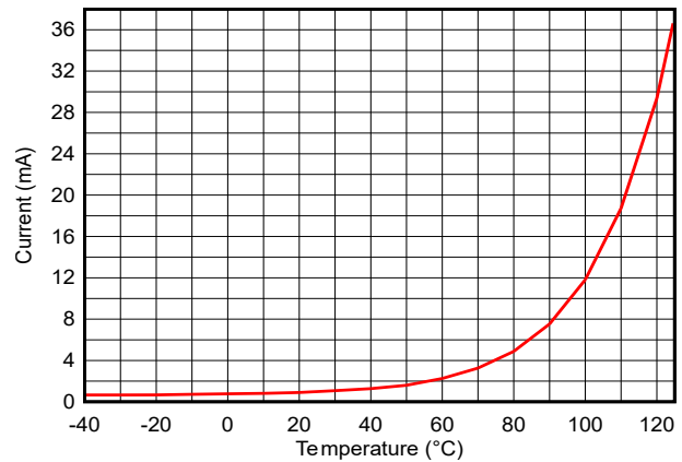
Figure 7-7. Standby Mode (MCU) Current vs Temperature (SRAM and partial register retention, RTC enabled), V_{DD5} = 3.3\text{V}
