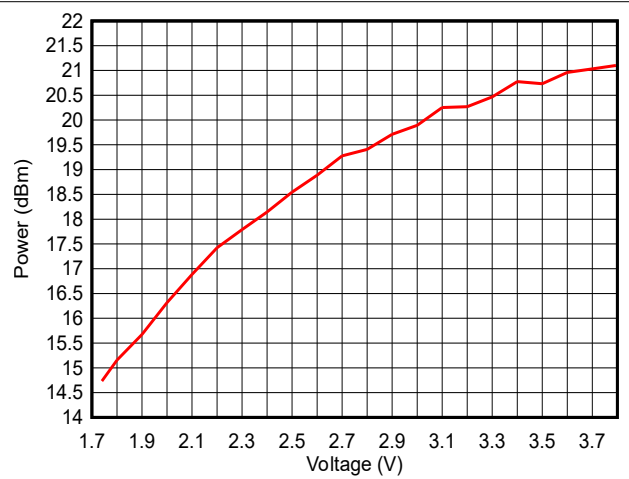
Figure 7-25. Output Power vs Supply Voltage (VDD5) (LE 1M PHY, 2.44GHz, +20dBm)
