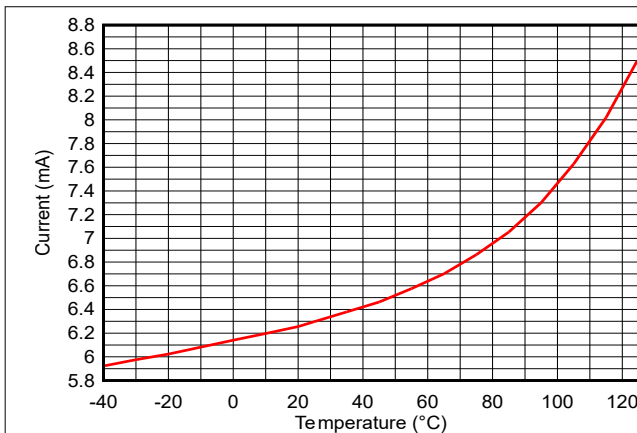
Figure 7-8. RX Current vs Temperature (LE 1M PHY, 2.44GHz), V_{DD5} = 3.3\text{V}
