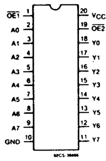
Figure 3-2. CDx4AC541, CDx4ACT541
