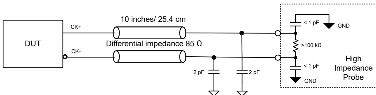
Figure 7-1. AC Test Load (Referencing Intel DB2000QL Document)
