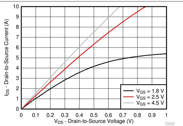
Figure 5-2. Saturation Characteristics
